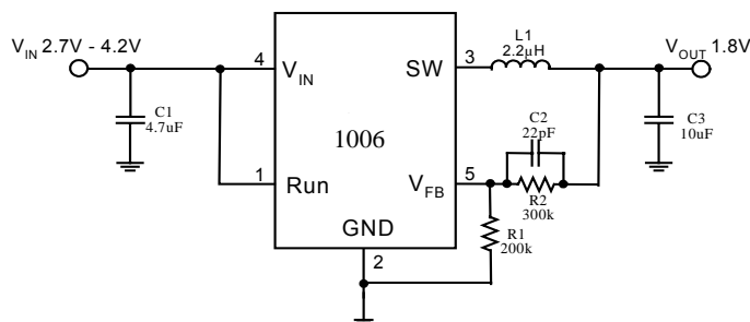
Figure 1. Basic Application Circuit with APS1006 adjustable version
