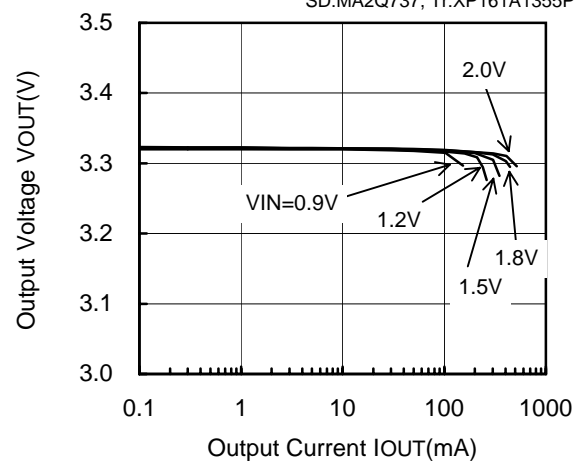
XC9104D092MR (PWM/PFM,180kHz,3.3V)
