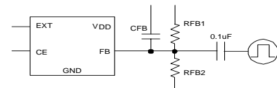
CIRCUIT ⑥
