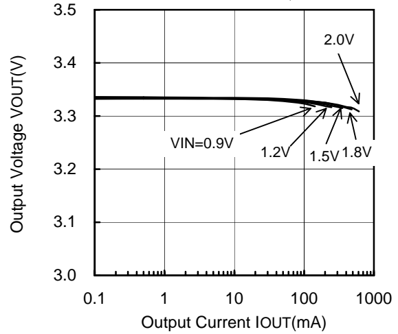
XC9104D095MR (PWM/PFM,500kHz,3.3V)
