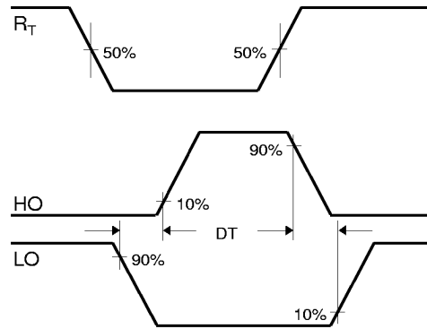
Figure 3. Deadtime Waveform Definitions
