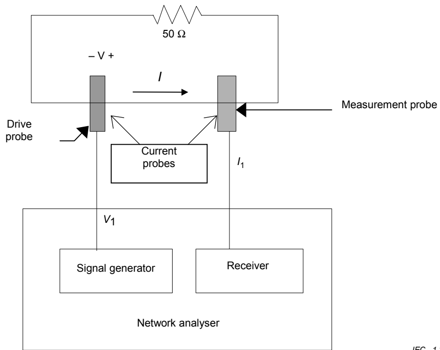
Figure C.5 – Calibration fixture
