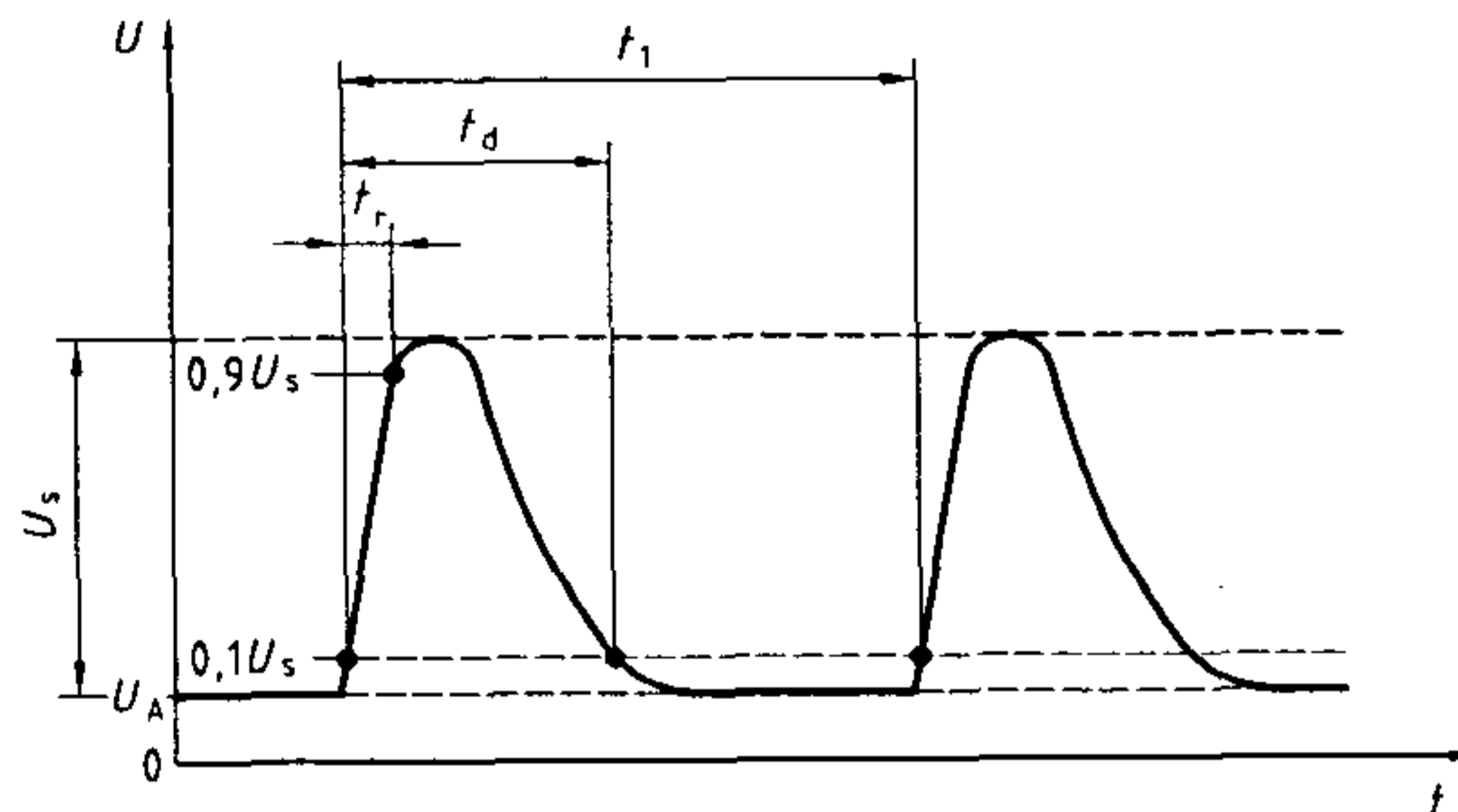
Figure 6 — Test pulse 2a
