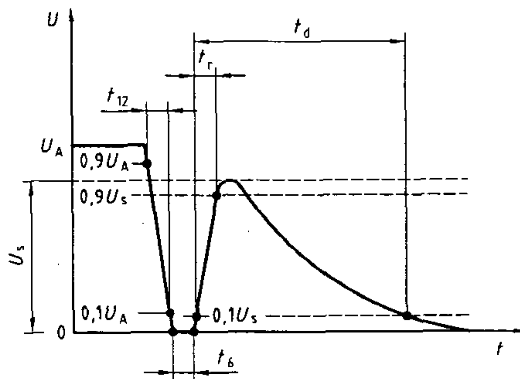
Figure 7 — Test pulse 2b
