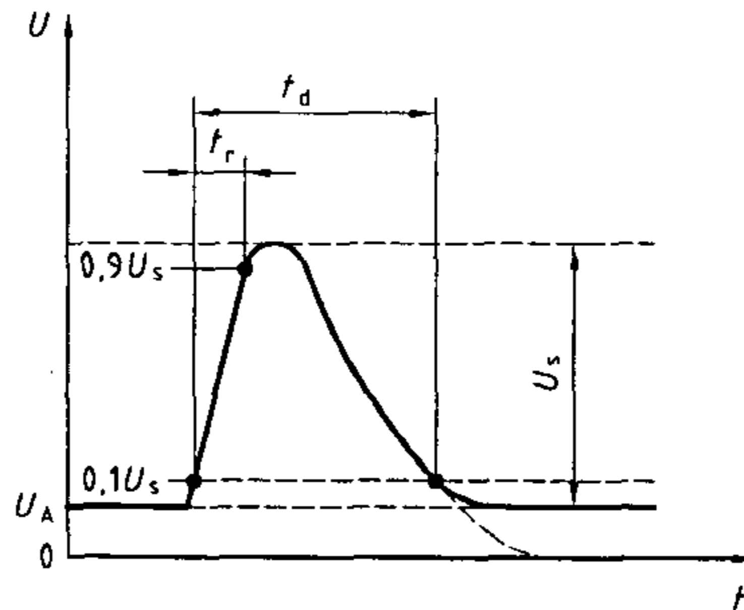
Figure 11 — Test pulse 5a
