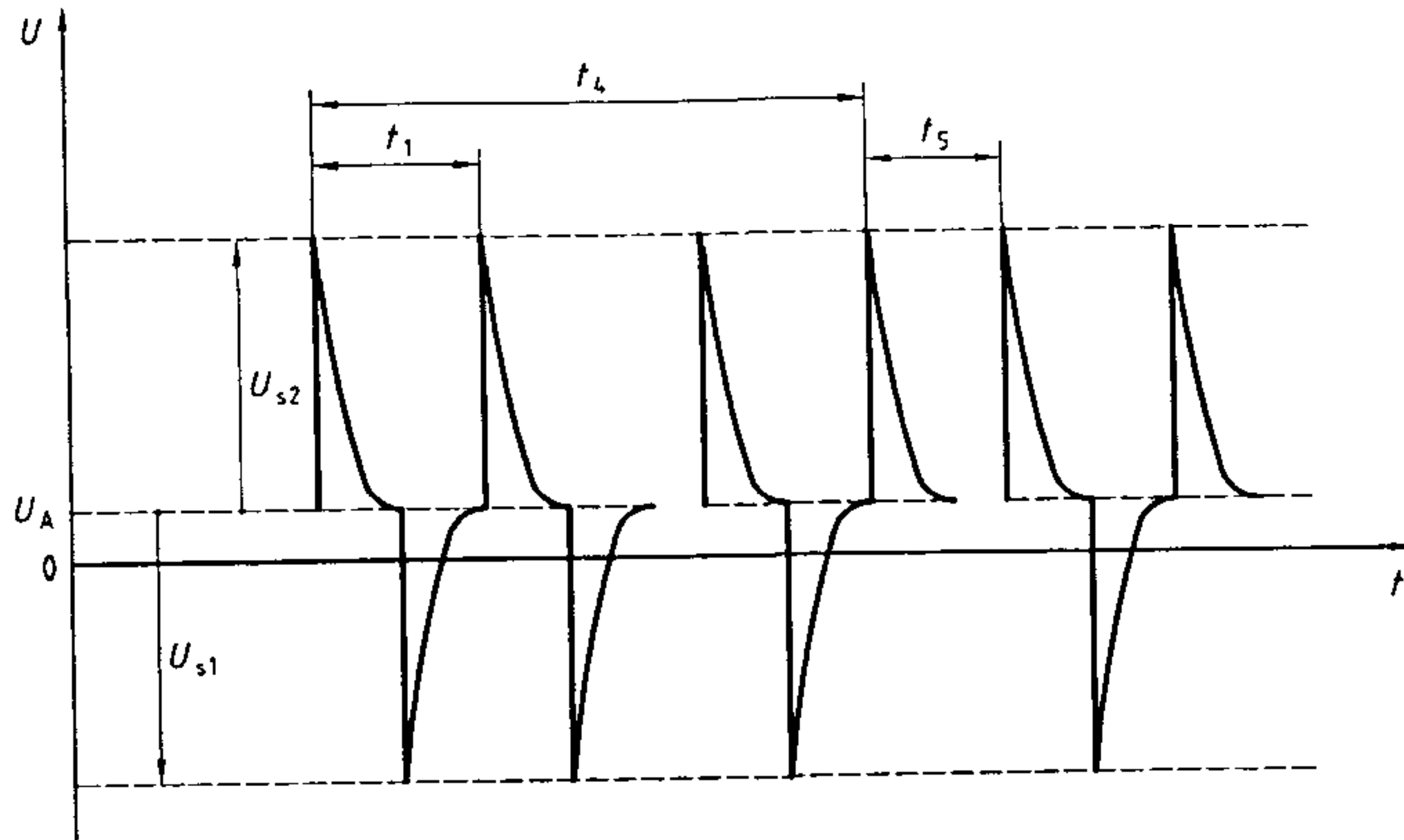
Figure C.2 — Burst transient waveform
