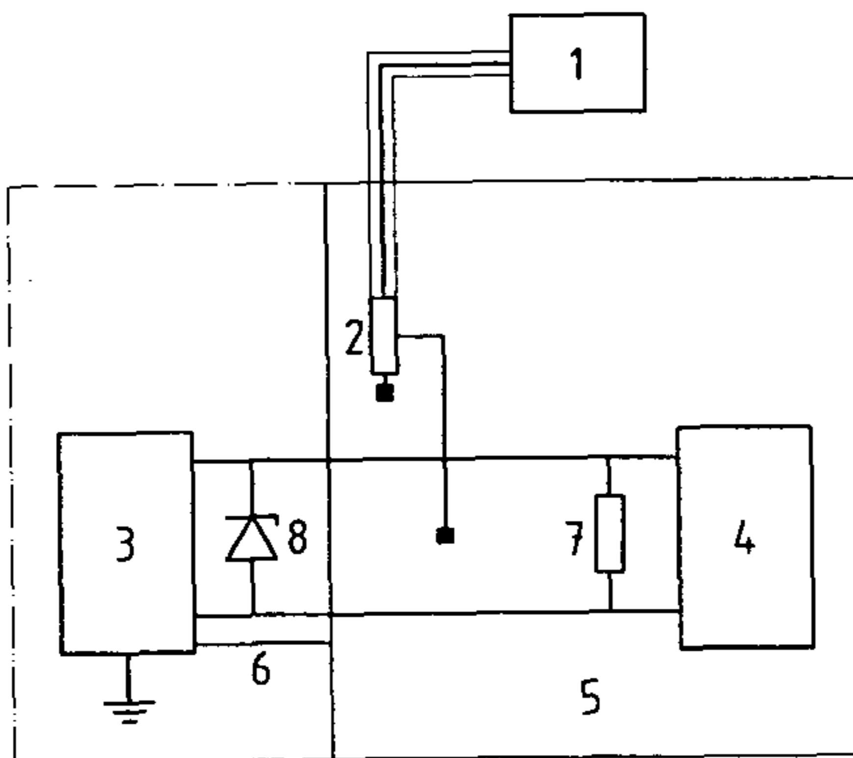
b) Pulse injection
