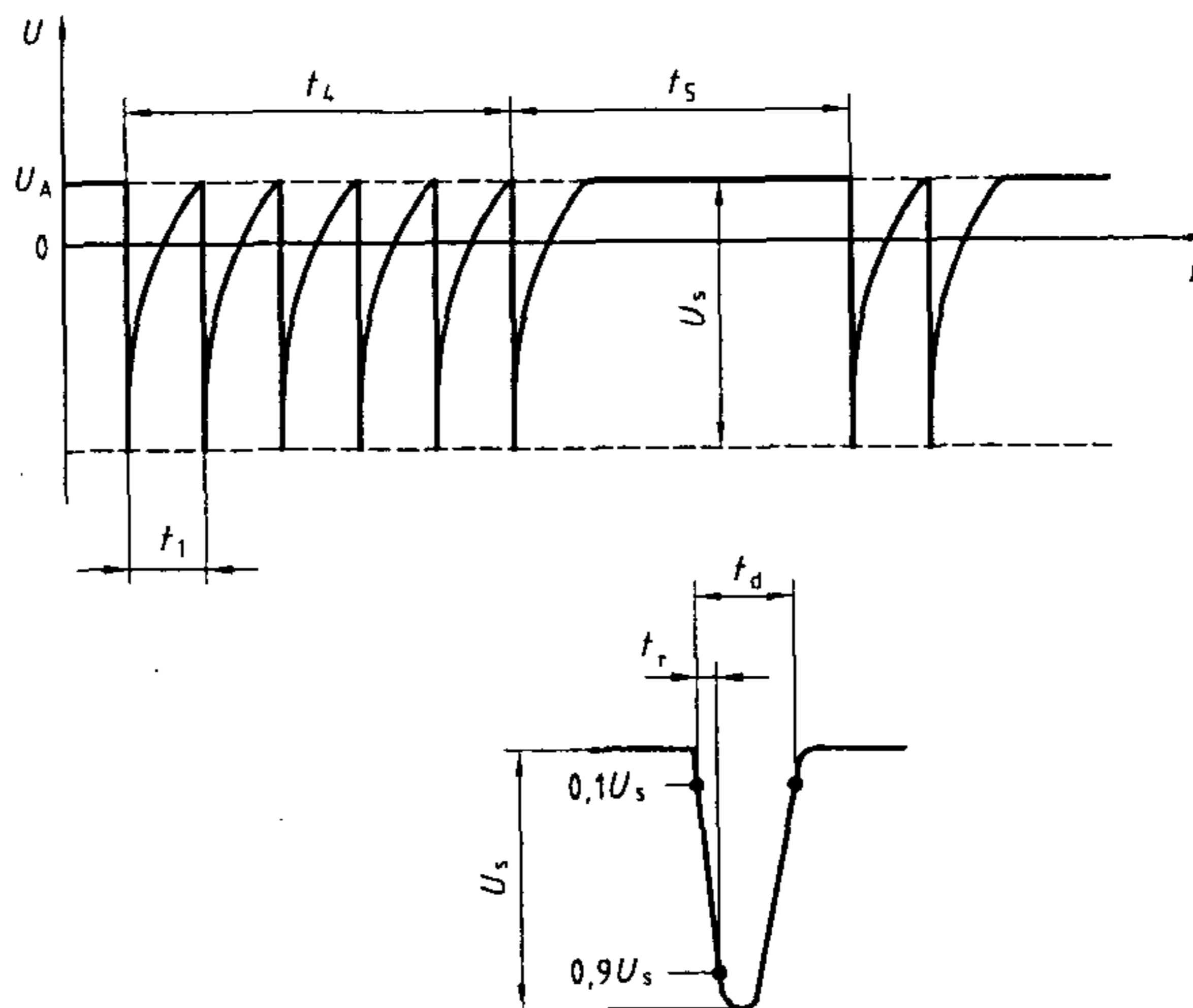
Figure 8 — Test pulse 3a
