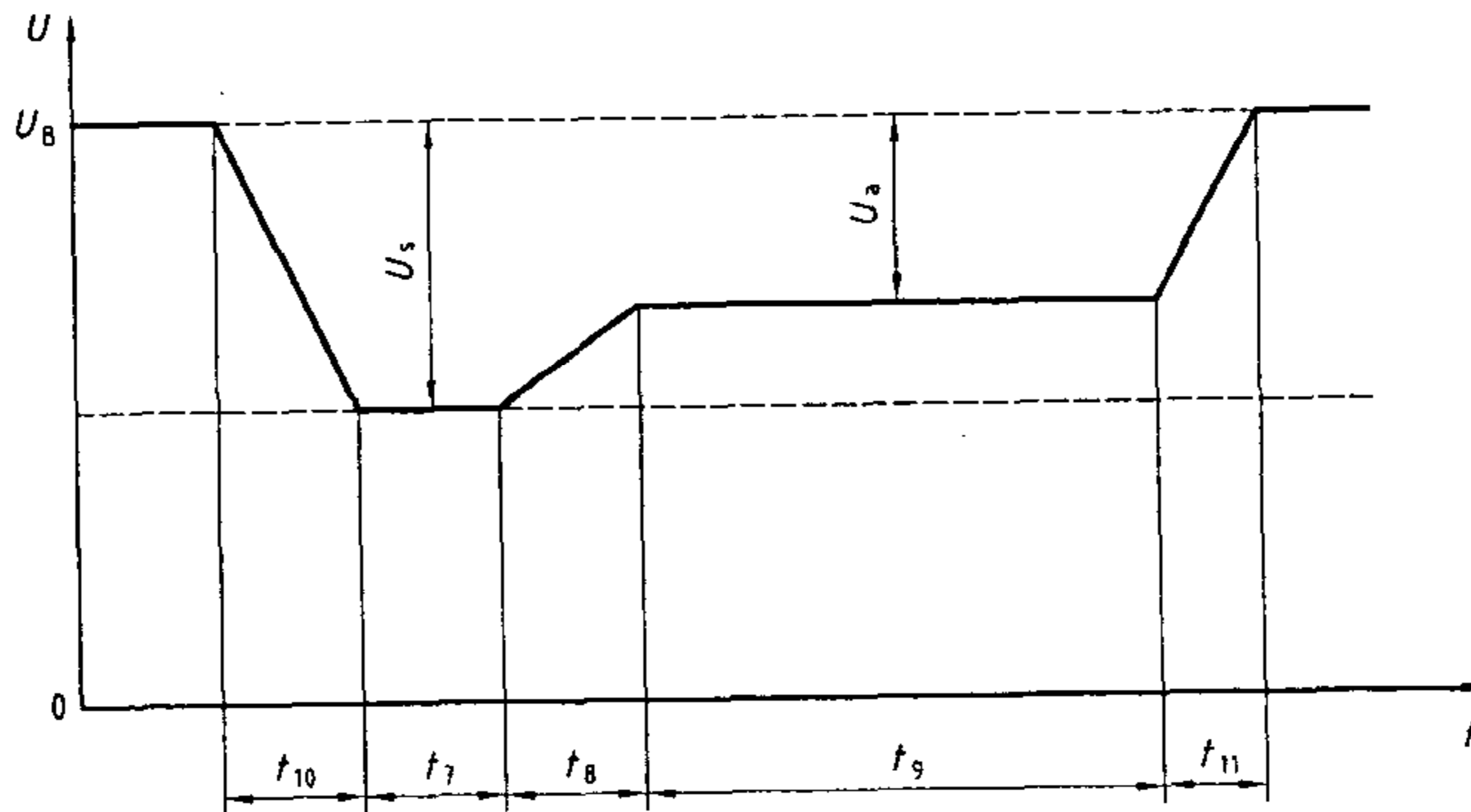
Figure 10 — Test pulse 4
