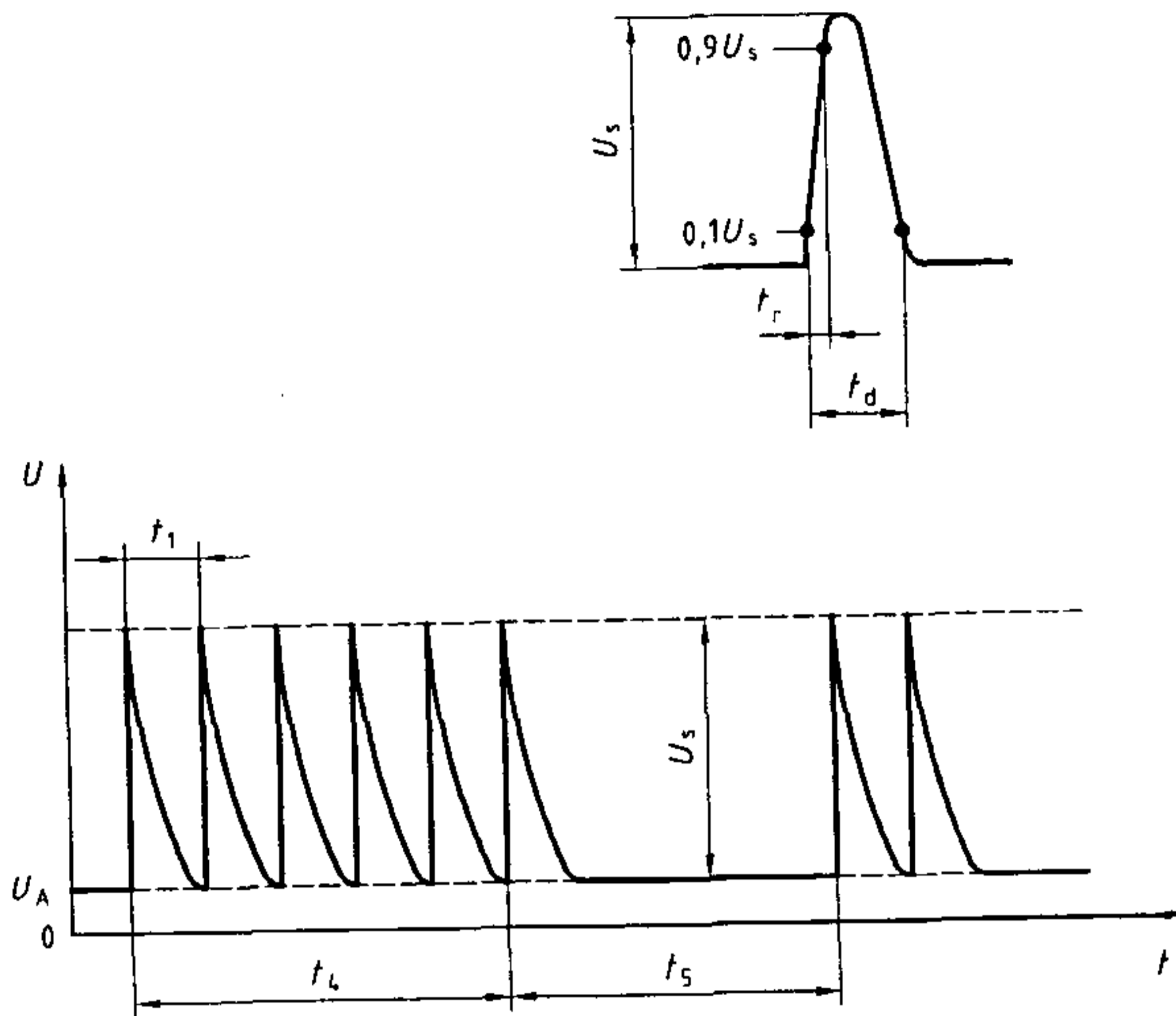
Figure 9 — Test pulse 3b
