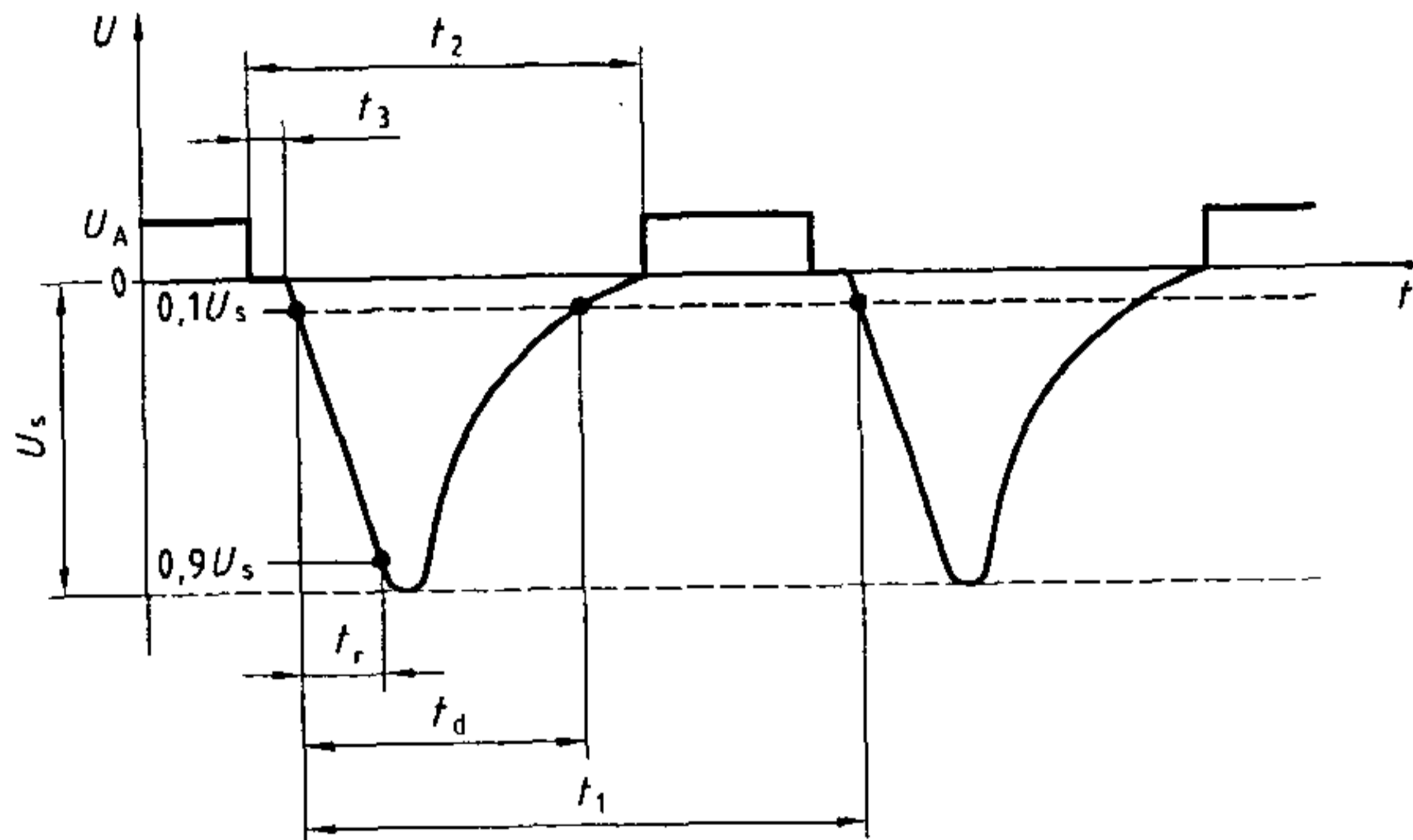
Figure 5 — Test pulse 1
