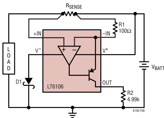
Figure 6. Schottky Diode Prevents Damage During Supply Reversal
