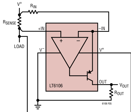
Figure 5. LT6106 Supply Current Monitored with the Load
