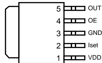
TO-252-5L
