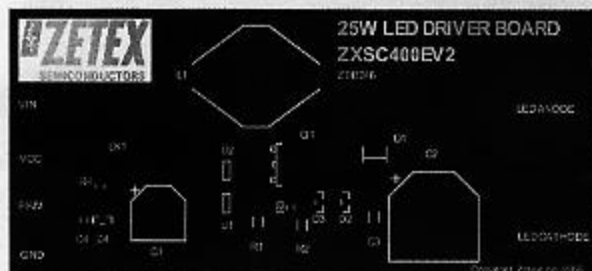
Top Silk
