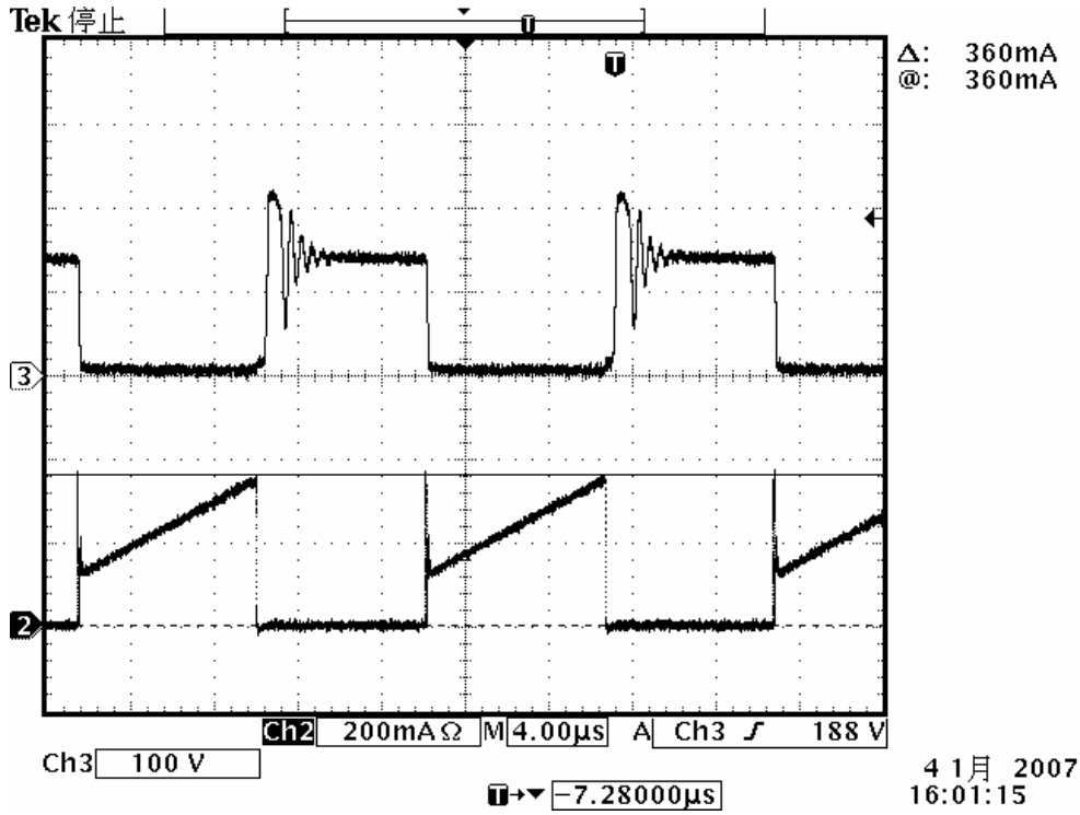
图 7, 85V 满载 (Ch3:Vc, Ch2:Ic)
