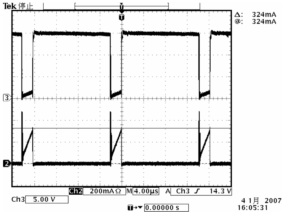
图 9, 85V 满载(Ch3:Ve, Ch2:Ic)
