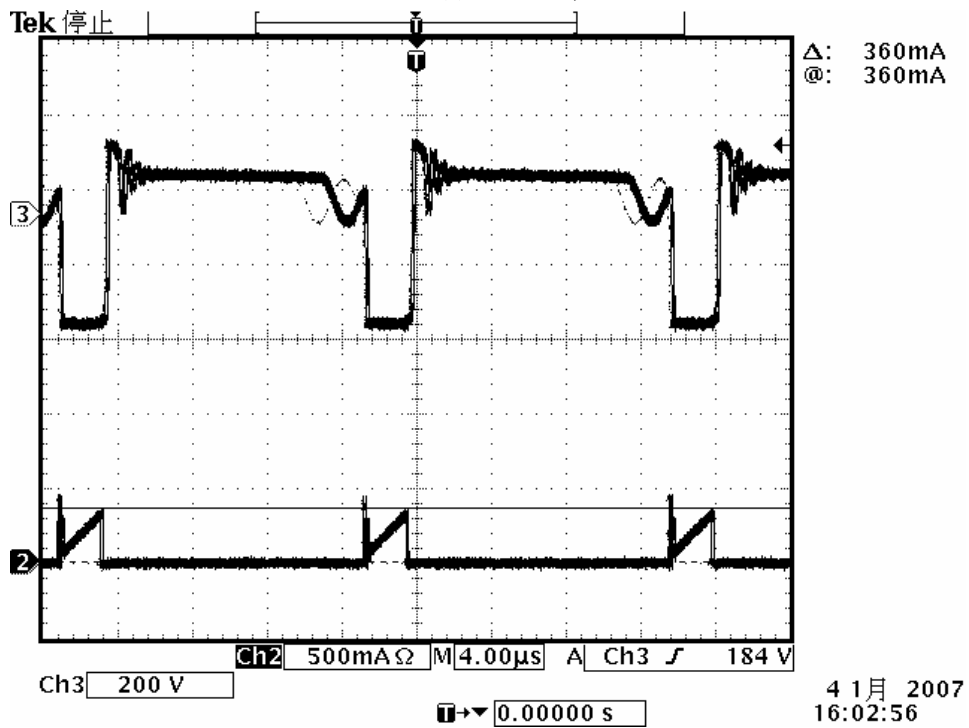
图 8, 264 V 满载 (Ch3:Vc, Ch2:Ic)
