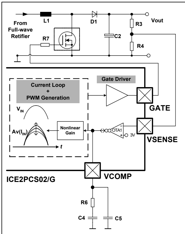
Figure 13 Voltage Loop
