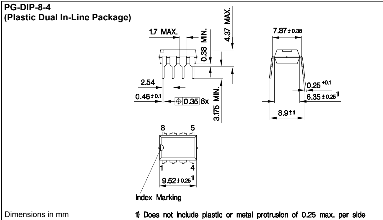
Figure 15 PG-DIP-8-4 Outline Dimension
