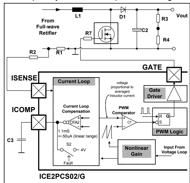
Figure 9 Complete System Current Loop
