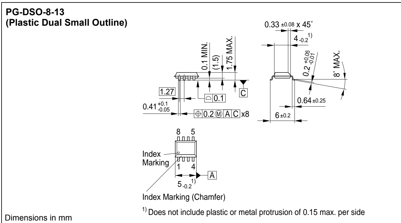
Figure 16 PG-DSO-8-13 Outline Dimension
