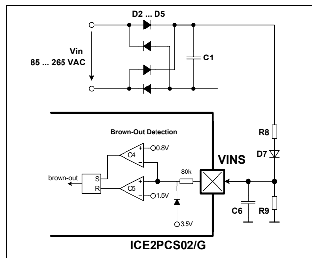
Figure 7 Input Brown-Out Protection (IBOP)
