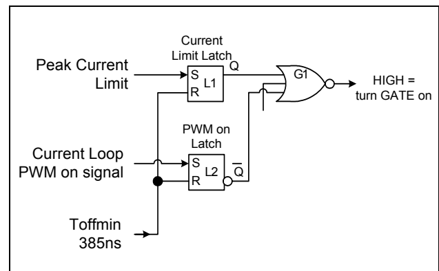
Figure 12 PWM Logic
