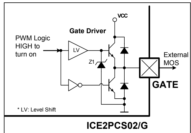
Figure 14 Gate Driver
