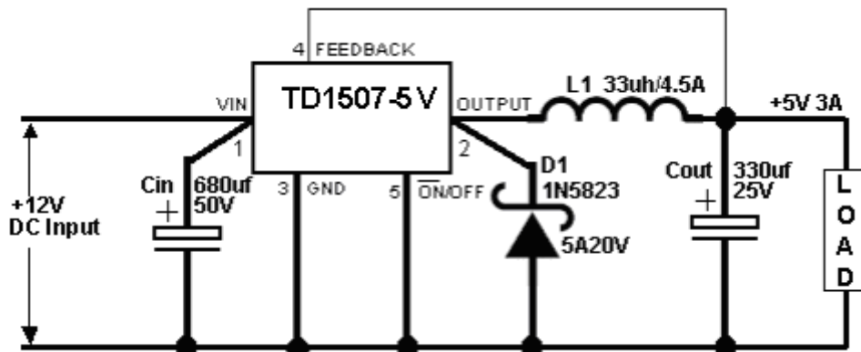
Figure 11. Typical Application of TD1507
