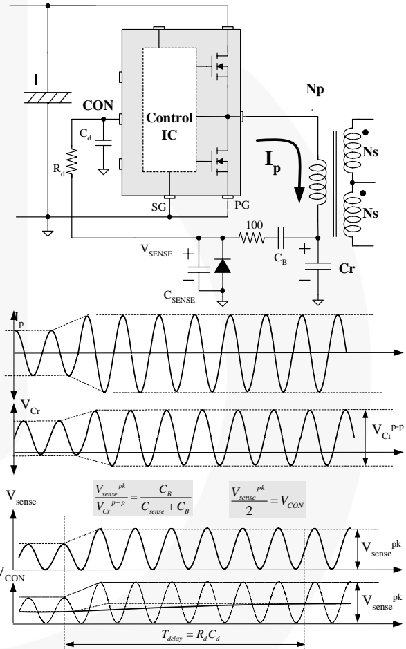
Figure 27. Current Sensing Using Resonant Capacitor Voltage
