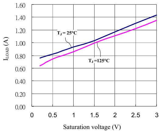
Saturation voltage vs. load current
