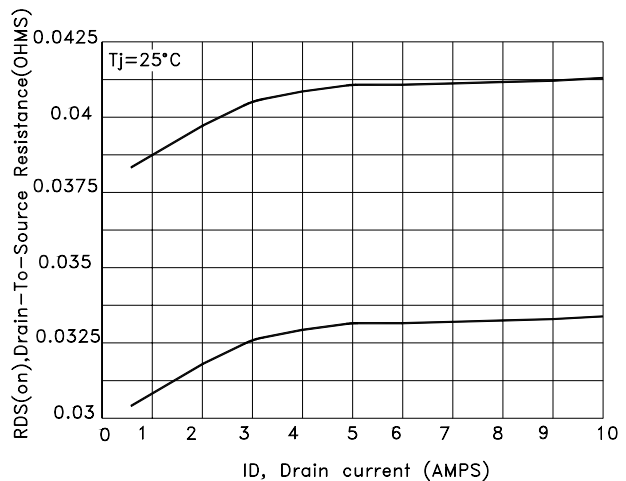
Fig.4 On-Resistance versus Drain Current and Gate Voltage
