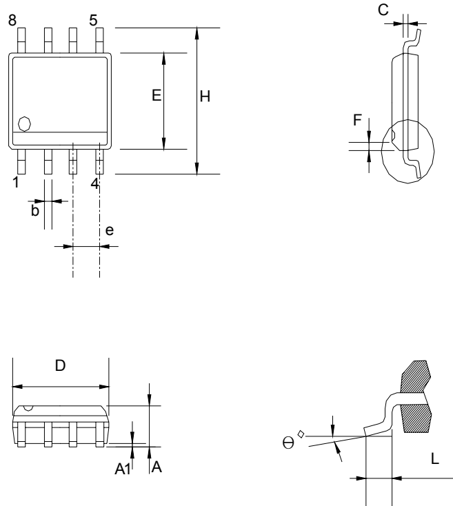
Figure 24. 8-SOP
