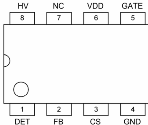
Figure 4. Pin Configuration
