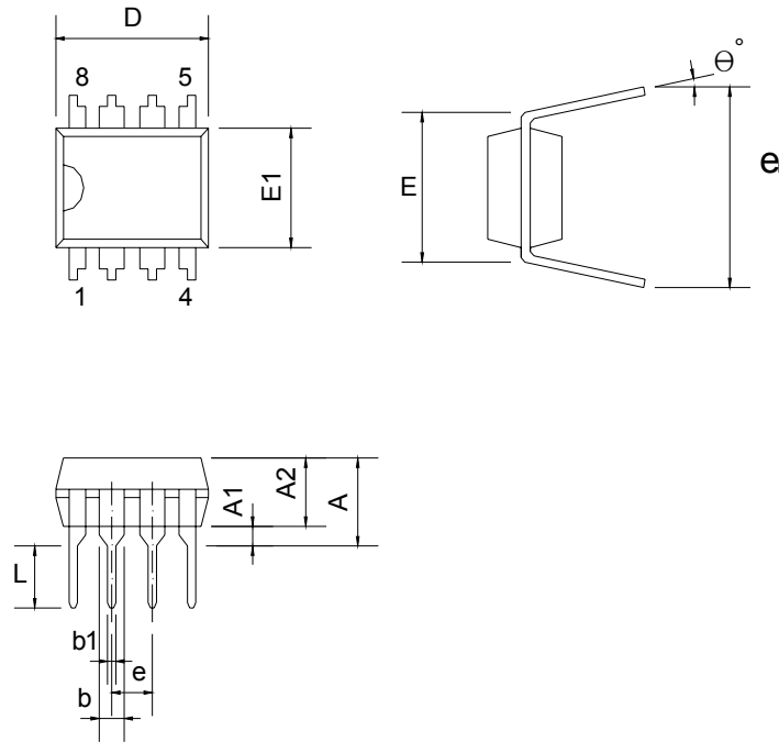
Figure 25. 8-DIP
