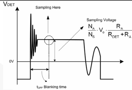
Figure 23. Voltage Sampled After 4μs Blanking Time After Switch-off Sequence
