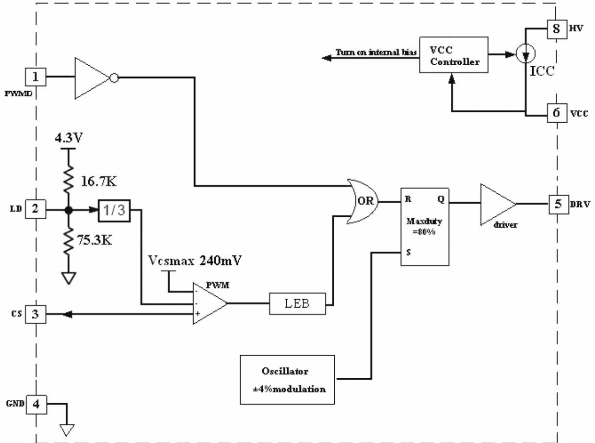
Figure 3. Block Diagram
