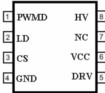
Figure 2. Pin Configuration (Top View)
