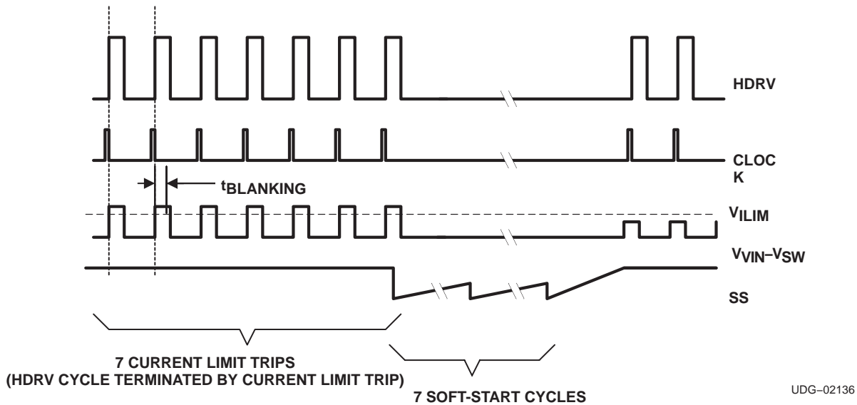
Figure 9. Typical Current Limit Protection Waveforms
