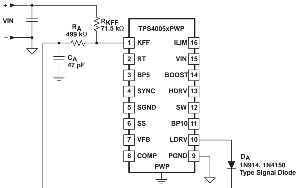
Figure 6. Hysteresis for Programmable UVLO
