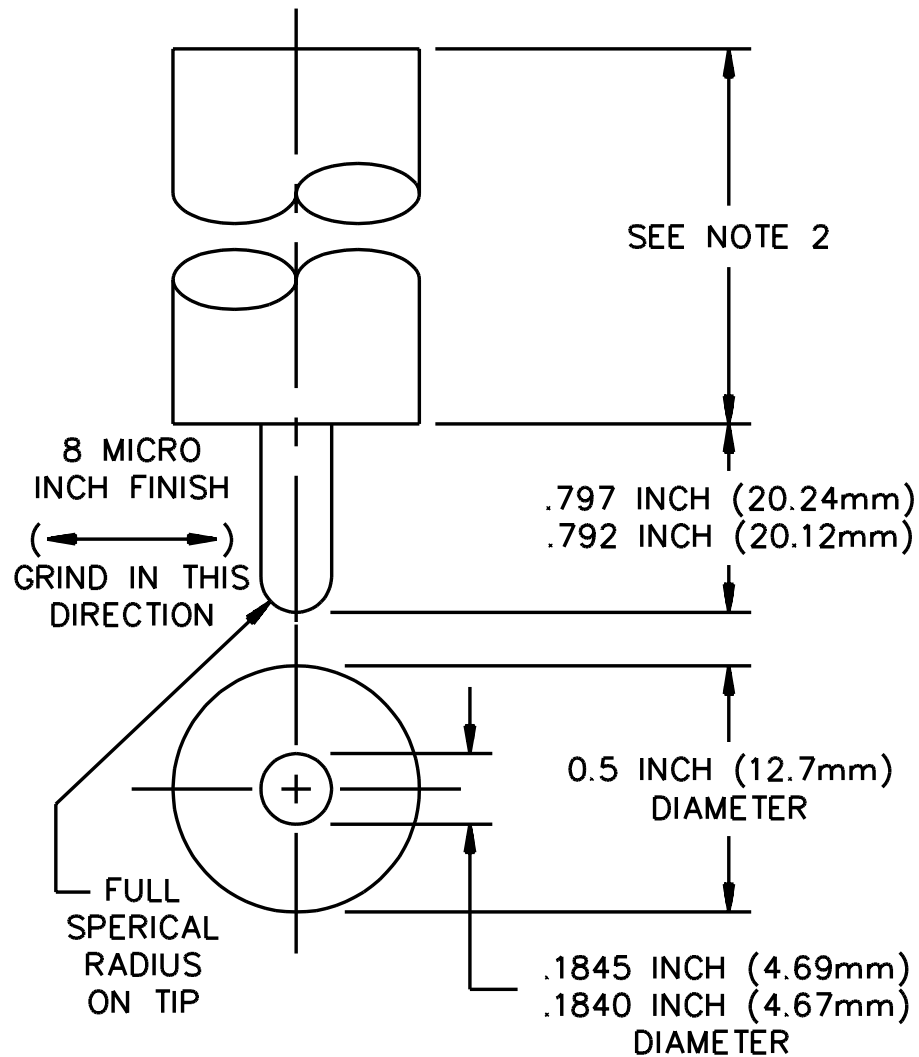
Figure SD5.1 Standard grounding pin
