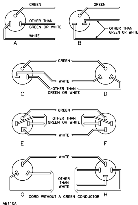
Figure 164.1 Identifying cord or lead connections
