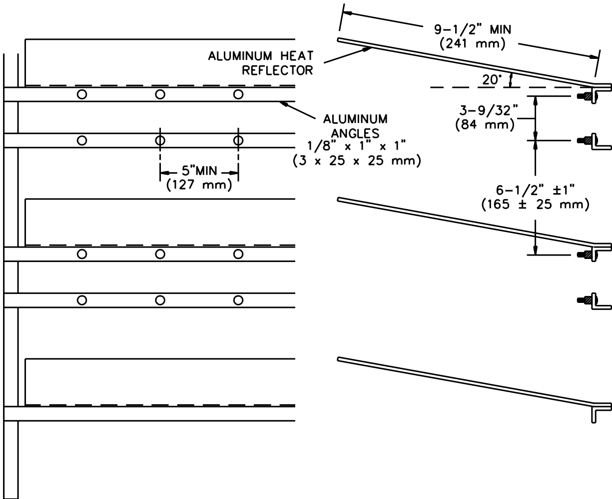
Figure 130.2 Test fixture
