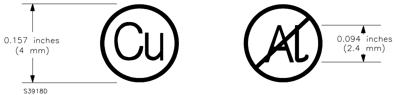
Figure 163.1 Non-CO/ALR marking
