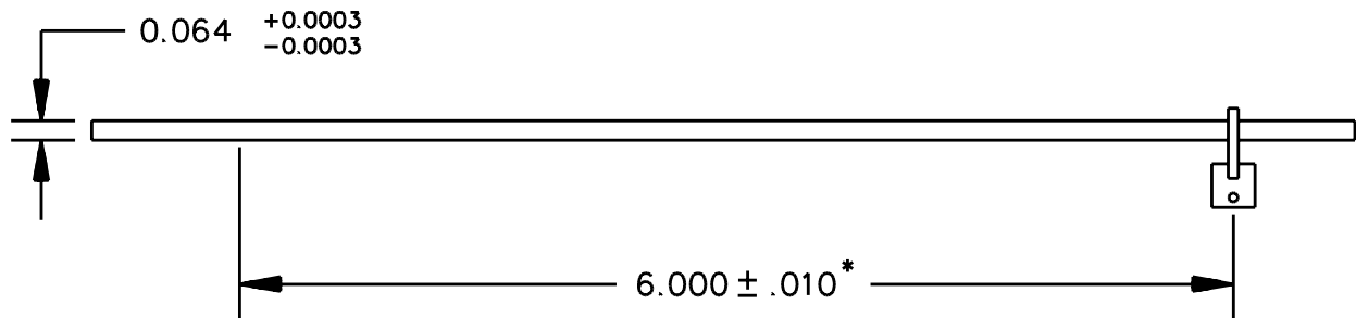
Figure 129.2 14 AWG test pin
