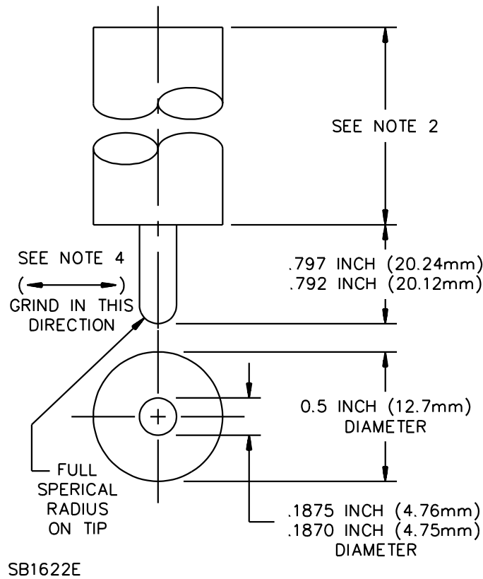
Figure 119.4 4 oz (113 g) ground pin
