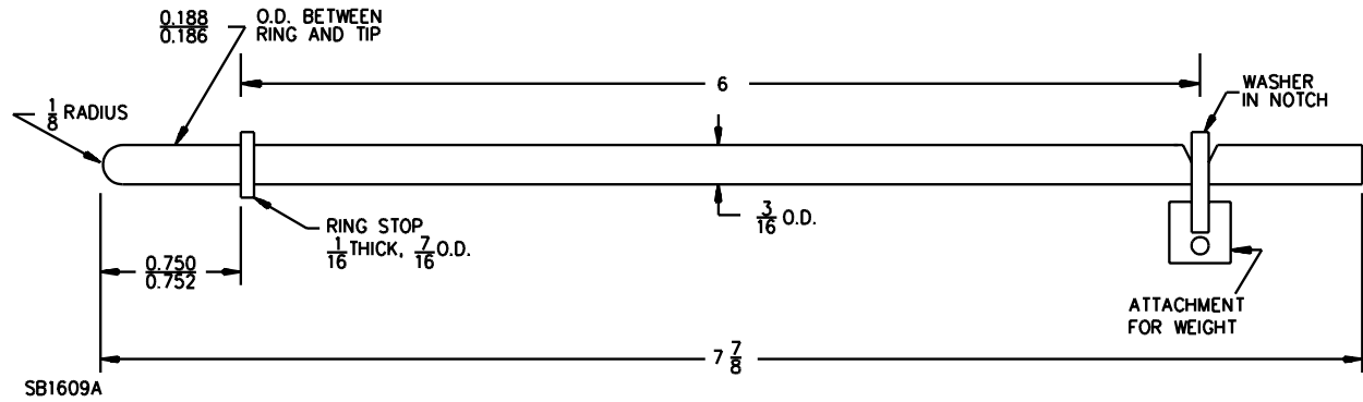
Figure 119.1 Test pin A
