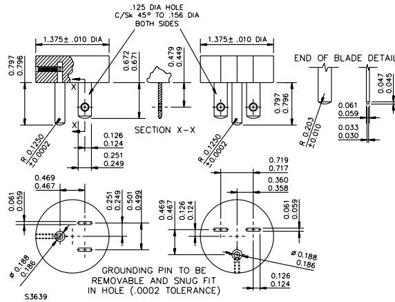
Figure 105.1 Test gauge
