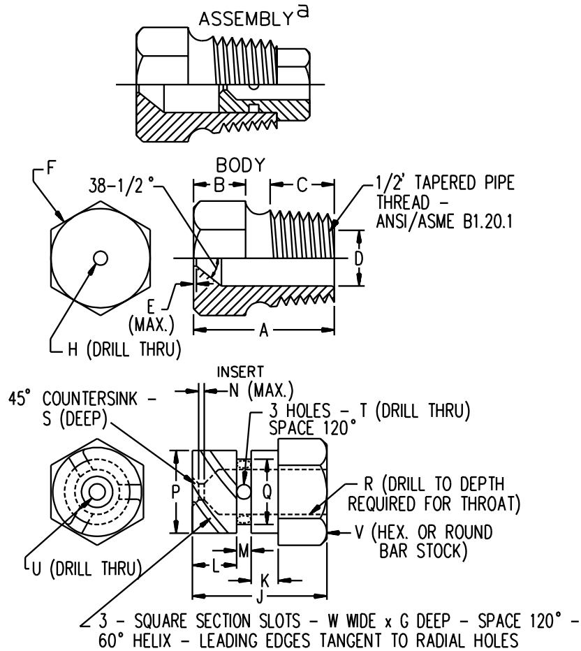
Figure SC11.2 Water-spray head
