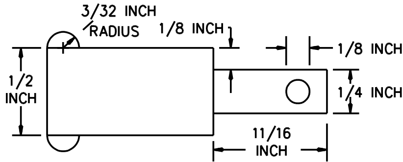
Figure 69.1 Reference plug
