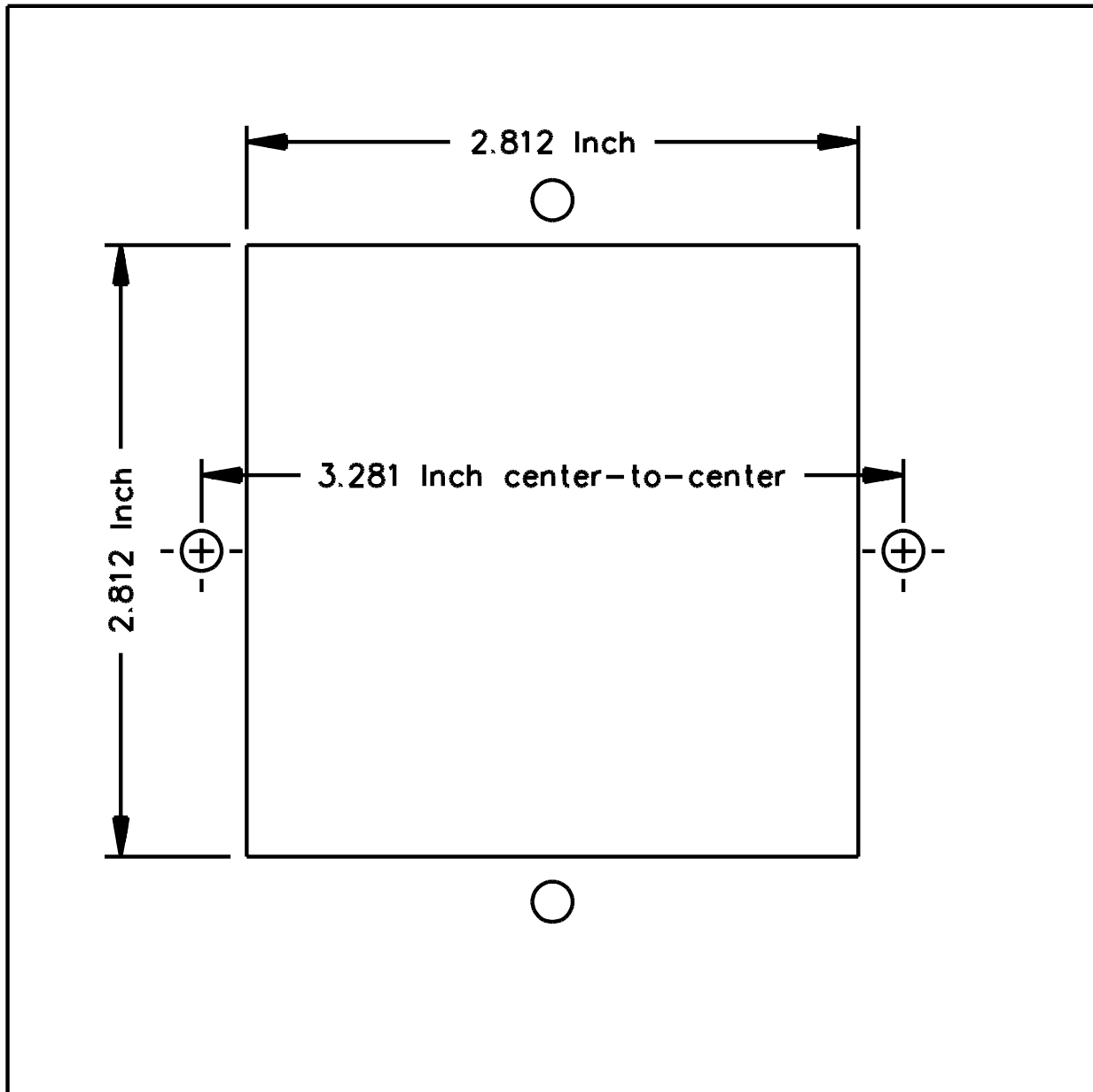
Figure 129.1 Test fixture
