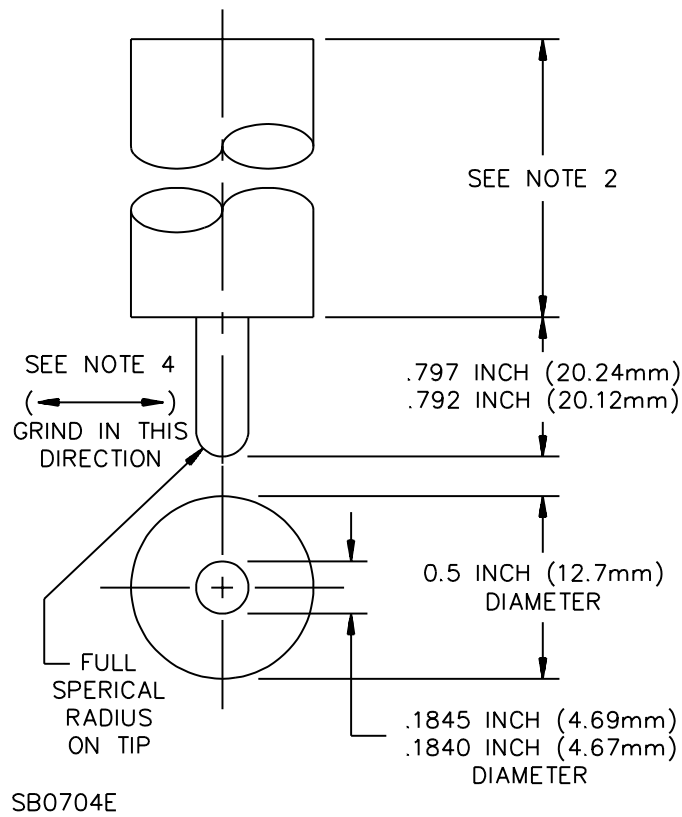
Figure 119.3 2 oz (57 g) ground pin
