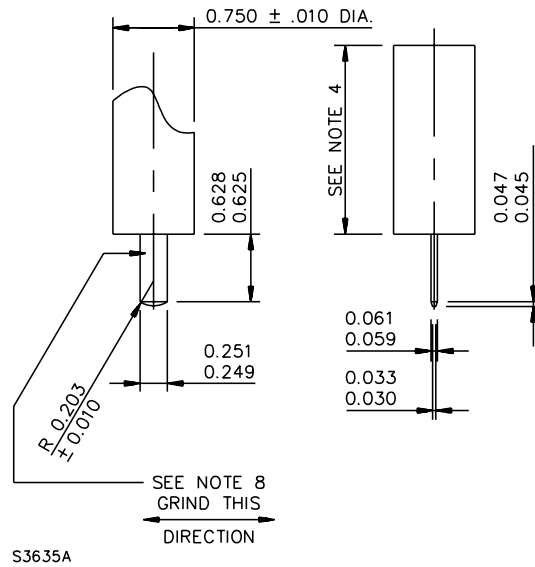
Figure 105.2 Test blade
