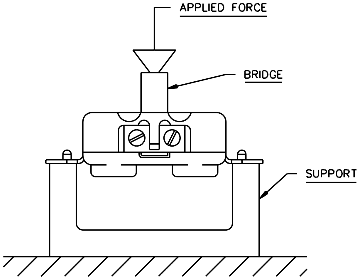
Figure 118.4 Assembly security test method (inverted)
