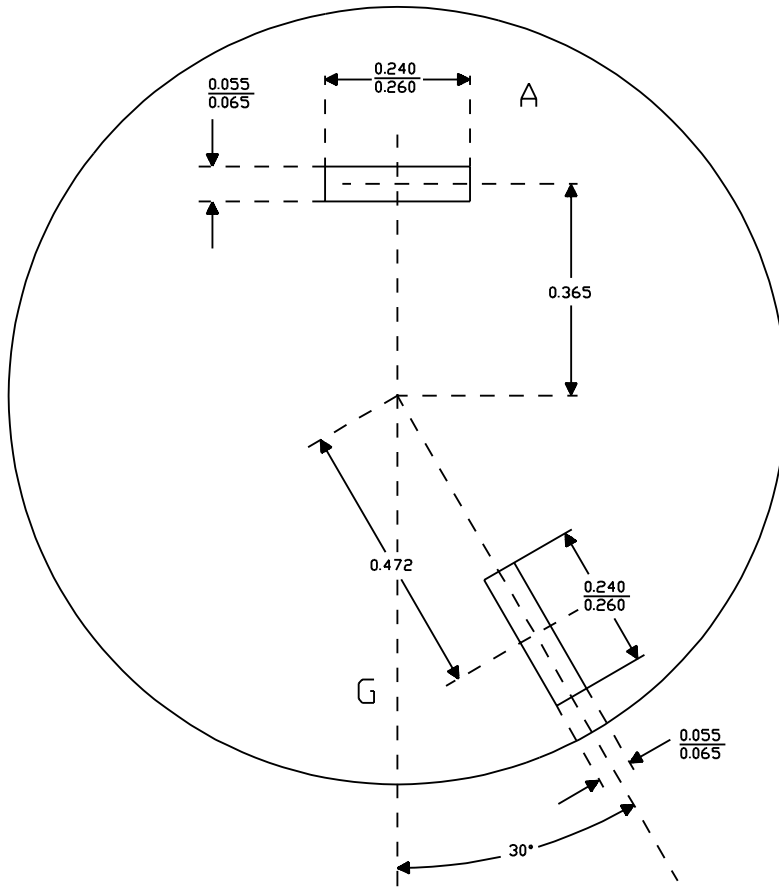
Figure 21.1 Example of a radio-antenna plug configuration
