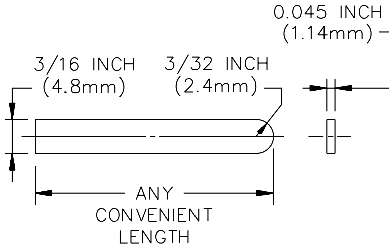
Figure 31.1 Flat probe
