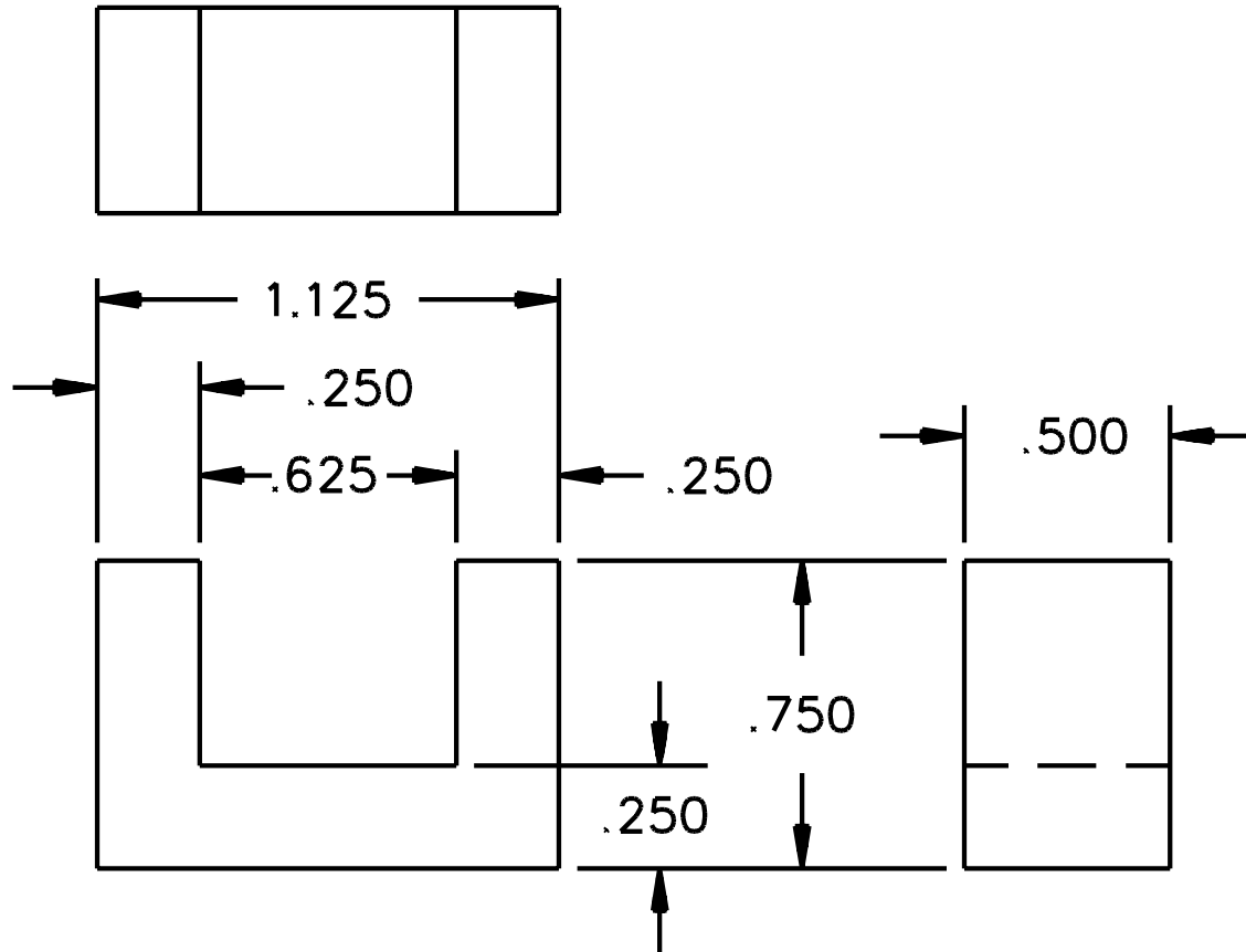
Figure 118.5 Bridge
