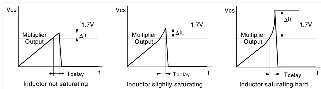
Figure 41. Effect of boost inductor saturation on the MOSFET current and detection method
