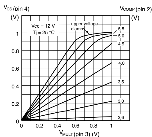
Figure 18. Multiplier characteristics @ V_{FF}=3V
