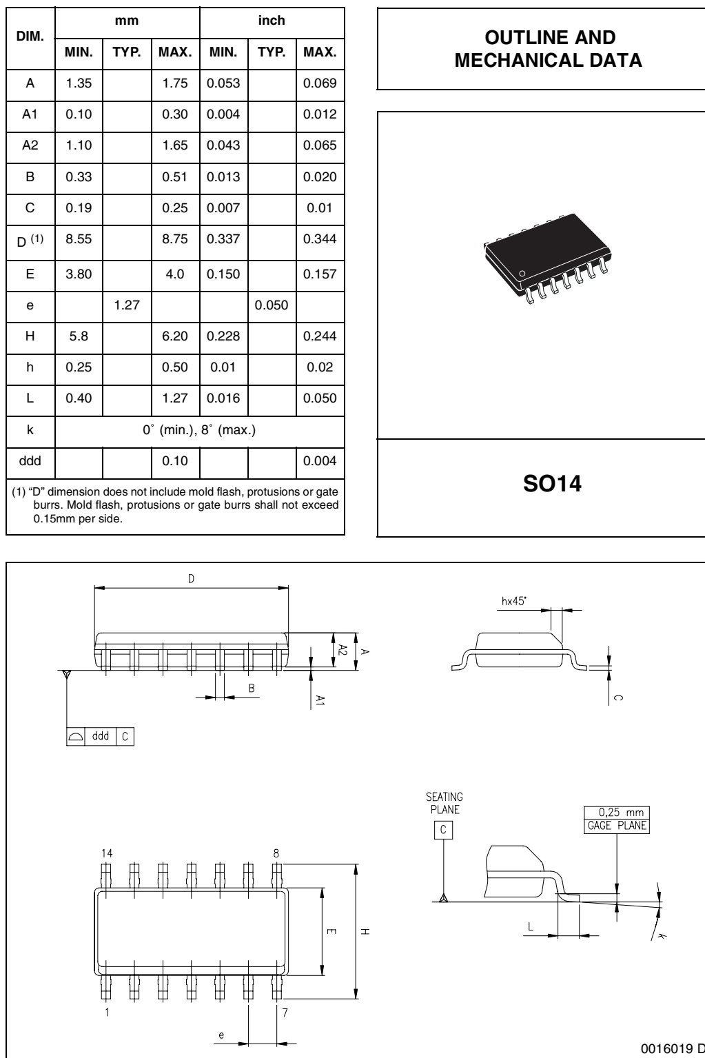
Figure 48. SO14 Mechanical Data & Package Dimensions
