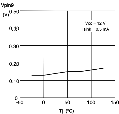
Figure 28. PWM_STOP low saturation vs. Tj
