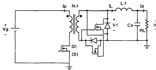
Fig. 7.- The intrinsic forward converter of the FAC
