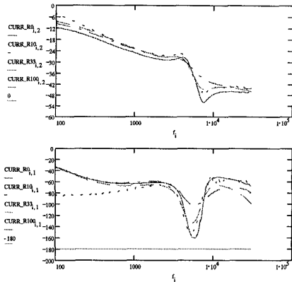
Fig. 15.-Comparison between FAC with different series resistors. The legend indicates the resistor value (ie. CURR_R33 means 33 Ohm ,current mode control)
