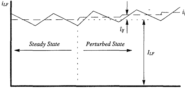
Fig. 2- Different components of the instantaneous current i_{LF} .
