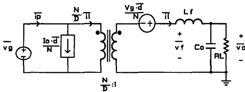
Fig. 5.- FAC equivalent small signal circuit
