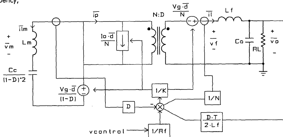
Fig. 12.- Small signal model of the FAC in peak current control mode to calculate the control to output transfer function.
