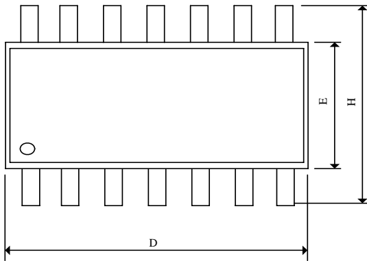
(e) 14 Pin SOP
