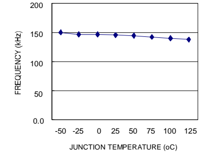
Switch Frequency
