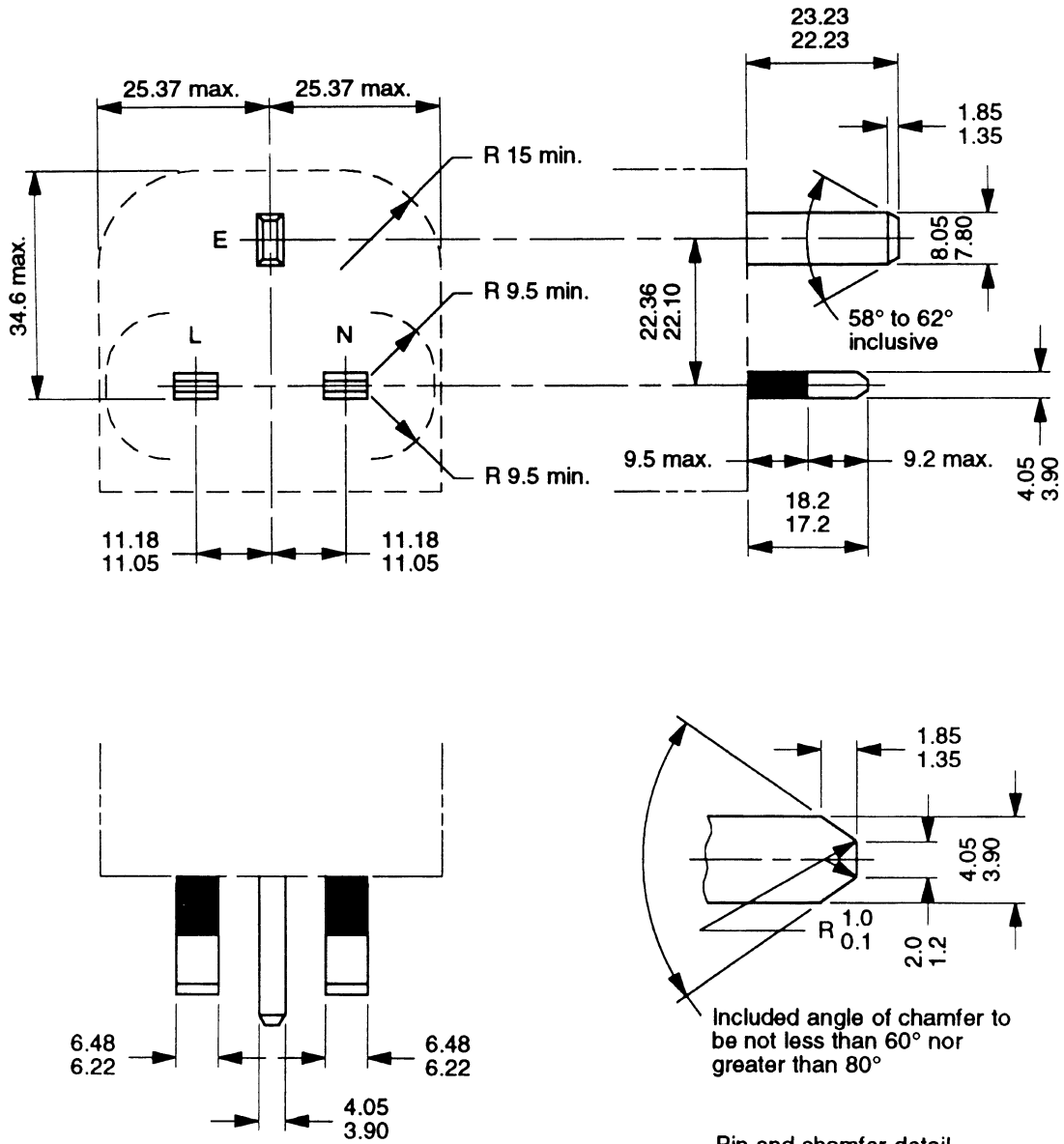
Figure 4 — Dimensions and disposition of pins (see clause 12)
