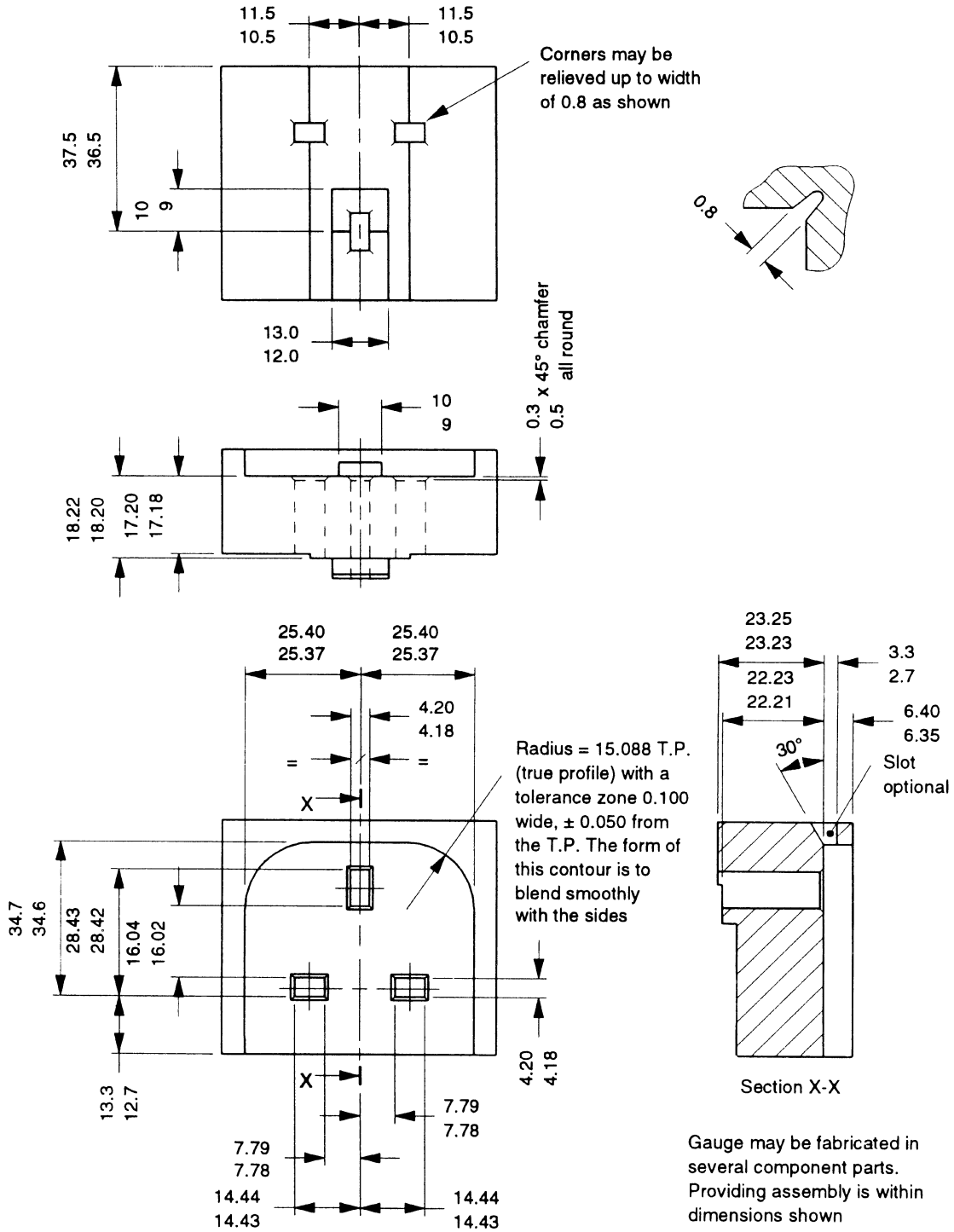
Figure 5 — Gauge for plug pins (see clauses 12, 20 and 22)
