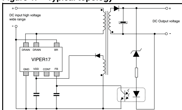
Figure 1. Typical topology
