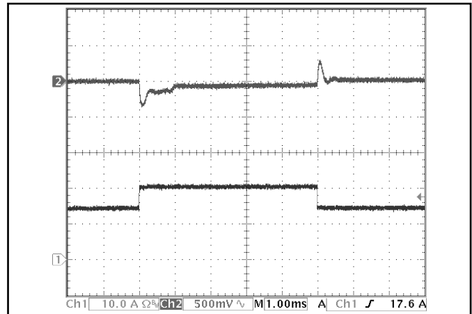
Figure 10: Output voltage response to step-change in load current (50%-75%-50% of I_{out(max)} ; dI/dt = 5A/\mu s ). Load cap: 470uF, 15 mΩ ESR tantalum capacitor. Top trace: Vout (500mV/div), Bottom trace: I_{out} (10A/div).
