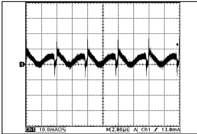
Figure 13: Input reflected ripple current, i_{sr} , through a 4.7\mu\text{H} source inductor, using a 100\mu\text{F} input capacitor, at nominal input voltage and rated load current (10 mA/div). See Figure 11.
