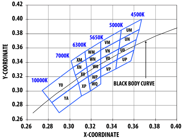
Figure 21. Color bin structure for Cool White.
