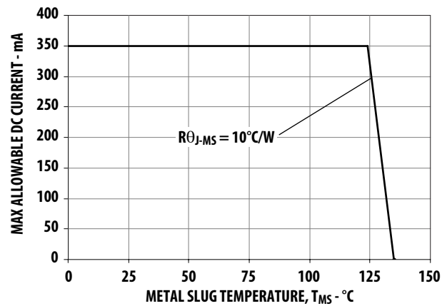
Figure 18: Maximum Forward Current vs. Metal Slug Temperature. Derated based on T_{JMAX} = 135^{\circ}C , R_{\theta J-MS} = 10^{\circ}C/W .
