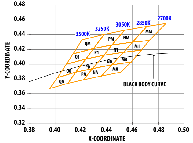
Figure 22. Color bin structure for Warm White.
