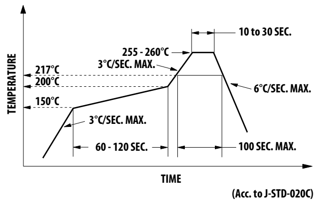
Figure 20. Recommended Reflow Soldering. (Acc. to J-STD-020C)
