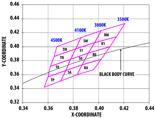
Figure 23. Color bin structure for Neutral White.
