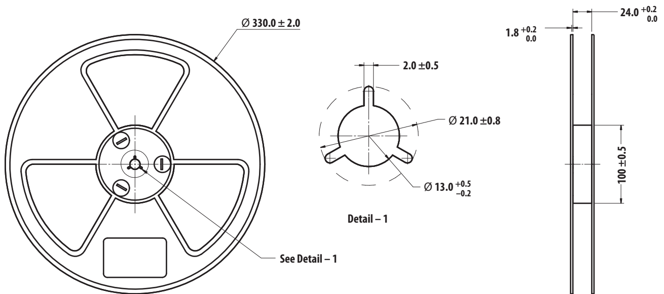
Figure 26. Reel dimensions.
