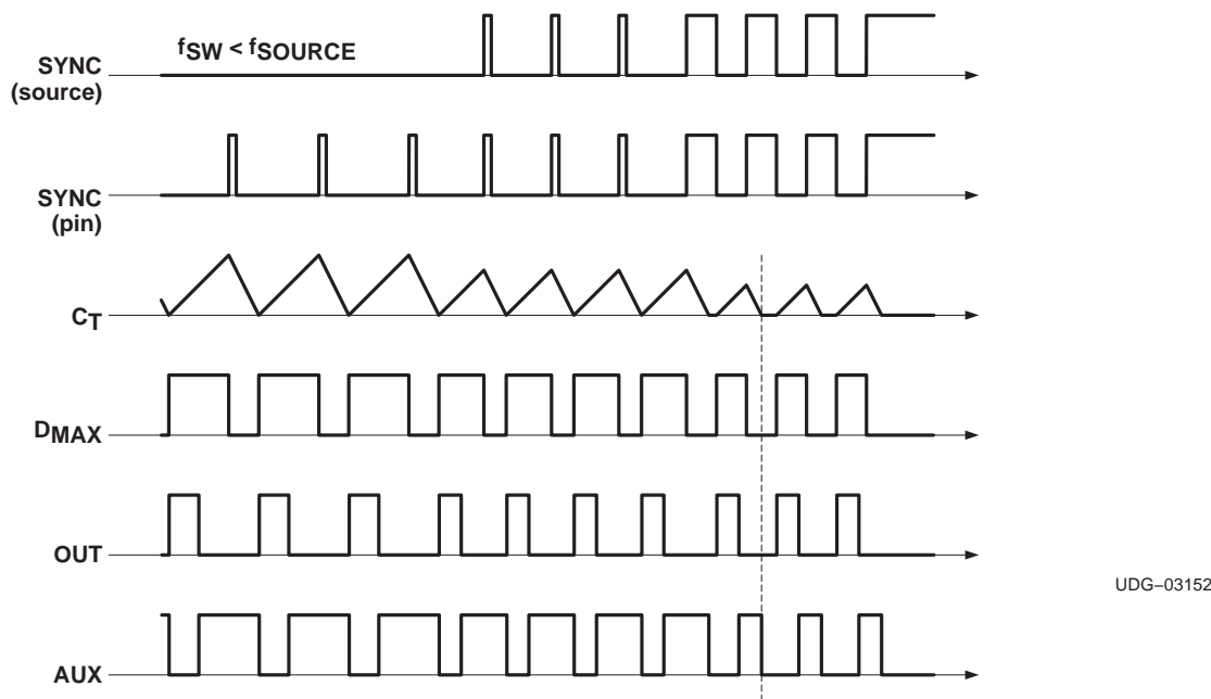
Figure 6. Synchronization Waveforms
