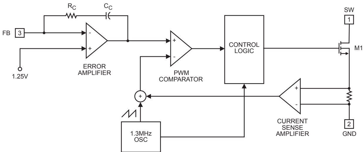
Figure 1—MP1541 Block Diagram
