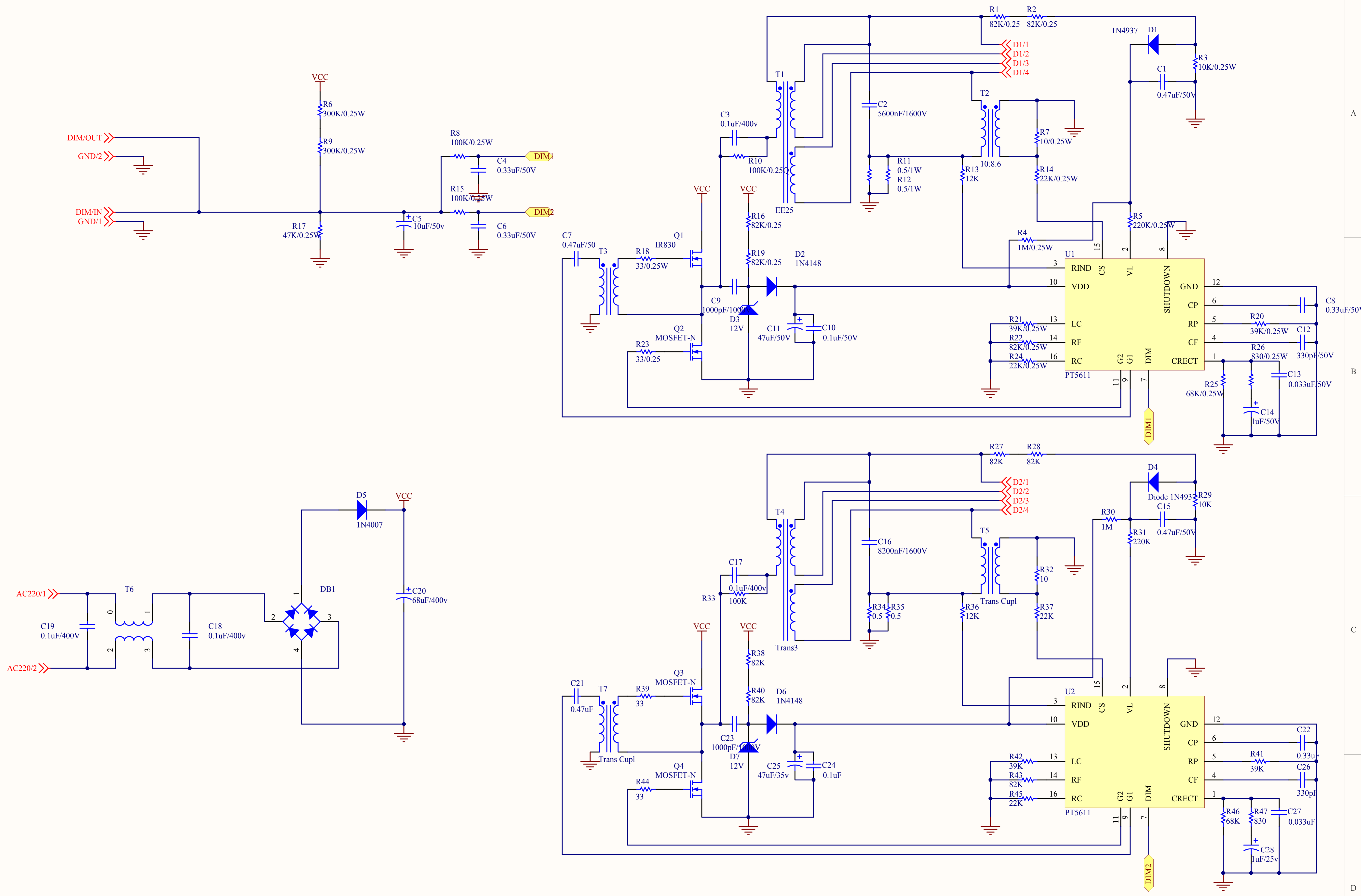
R4 R30 PCB
