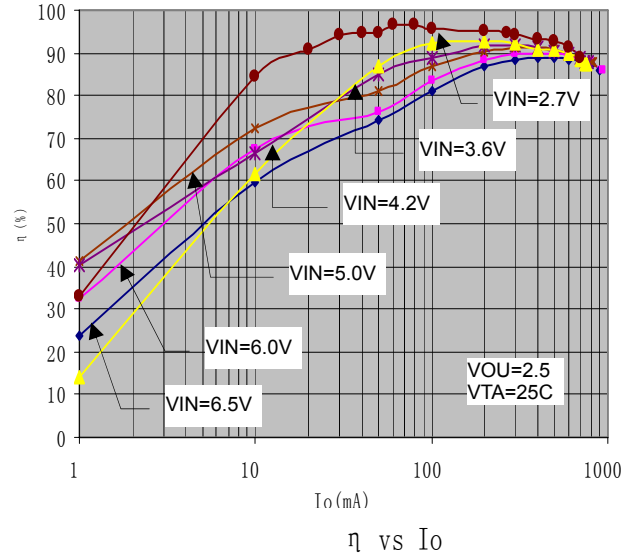
\eta vs I_o
