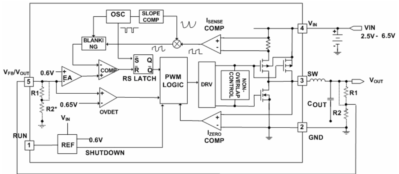
Figure 3. AP2406 Block Diagram
