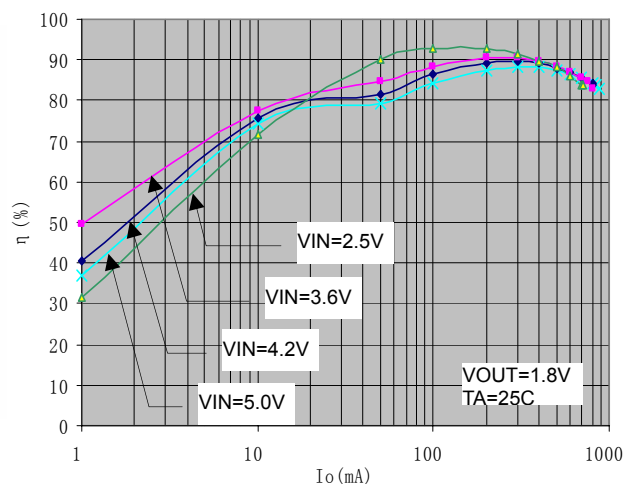
\eta vs I_o
