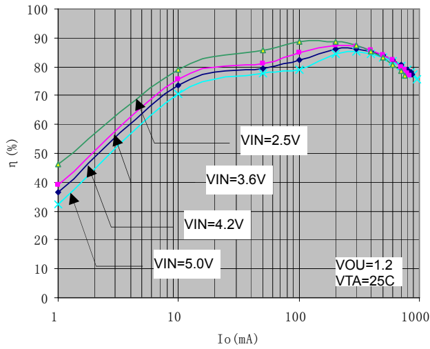
\eta vs I_o
