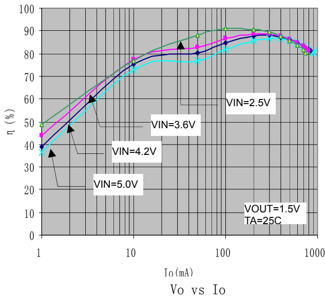
\eta vs I_o
