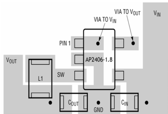
Figure5. AP2406 Fixed output Suggested Layout
