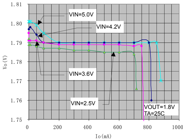
V_o vs I_o
