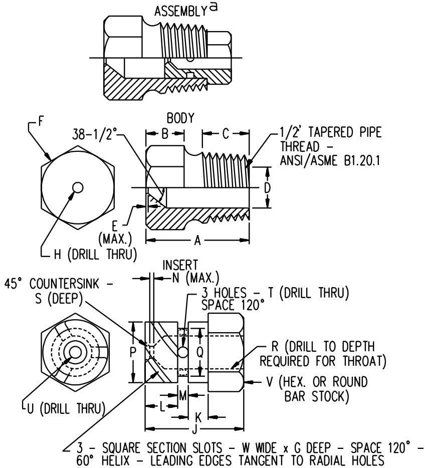
Figure 2 – Rain-test spray head
