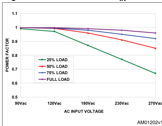
Figure 5. Power factor vs. V_{IN} and load
