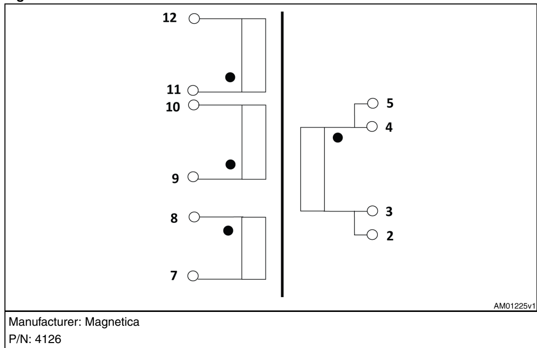
Figure 28. Power transformer
