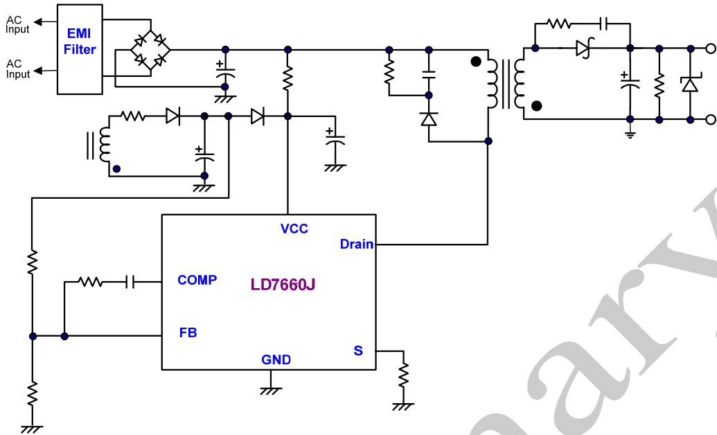
Primary-side Feedback
