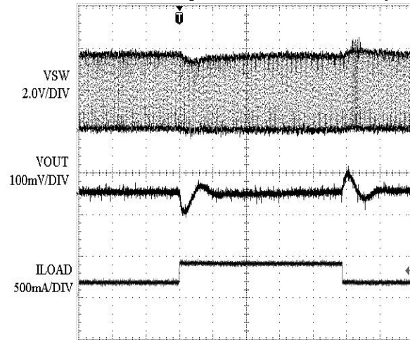
Load Transient Response PWM Mode Only
