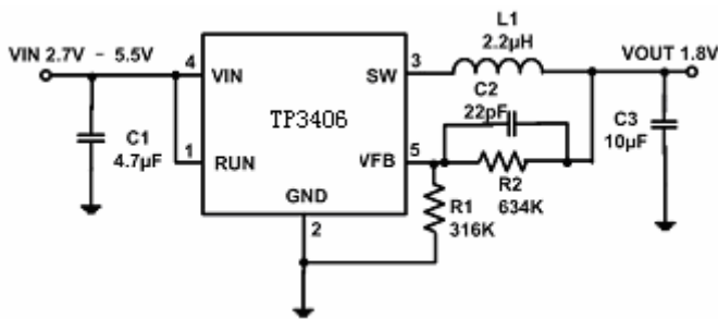
Figure 1. Basic Application Circuit with TP3406 adjustable version, V_{out} = 1.8V
