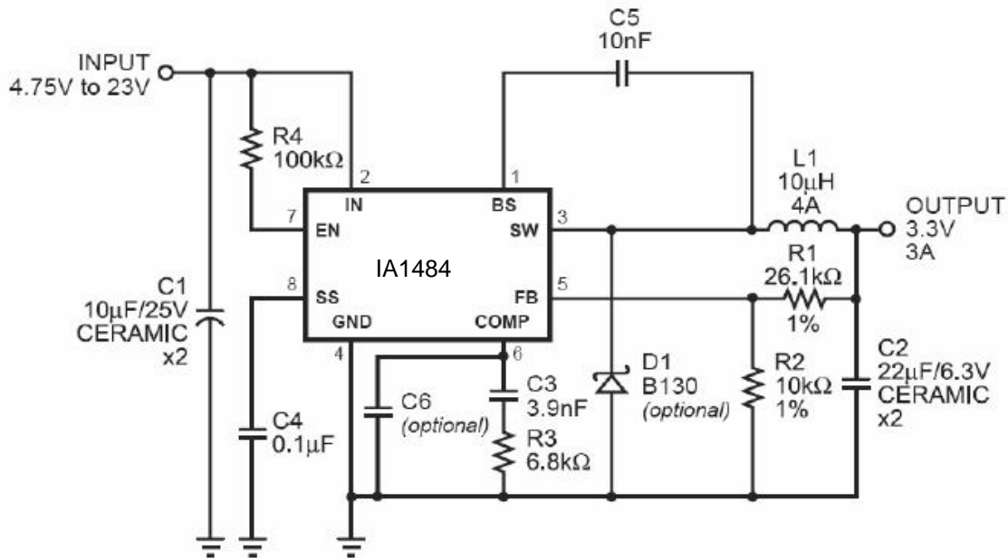
Figure 3- IA1484 with AVX 47µF, 6.3V Ceramic Output Capacitor
