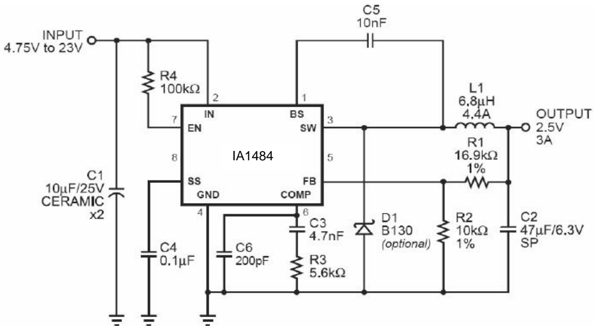
Figure 4- IA1484 with Panasonic 47µF, 6.3V Solid Polymer Output Capacitor
