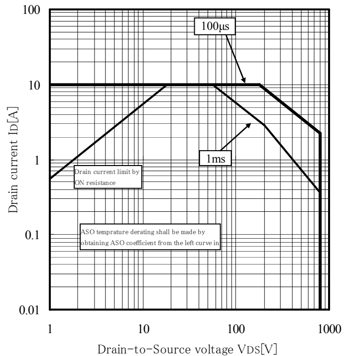
Fig3. MOSFET A.S.O.curve (Ta=25°C/Single Pulse)
