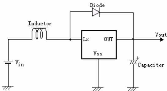
For use Build_in Transistor
