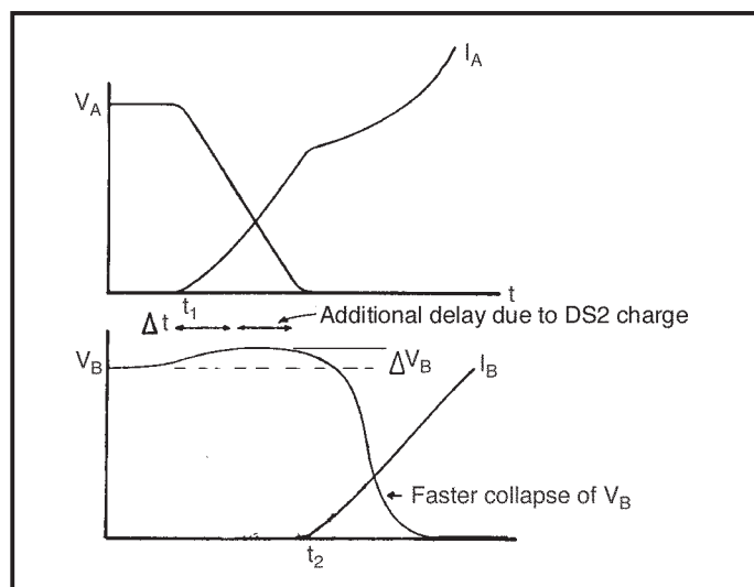
Fig. 2 Turn-on waveforms
