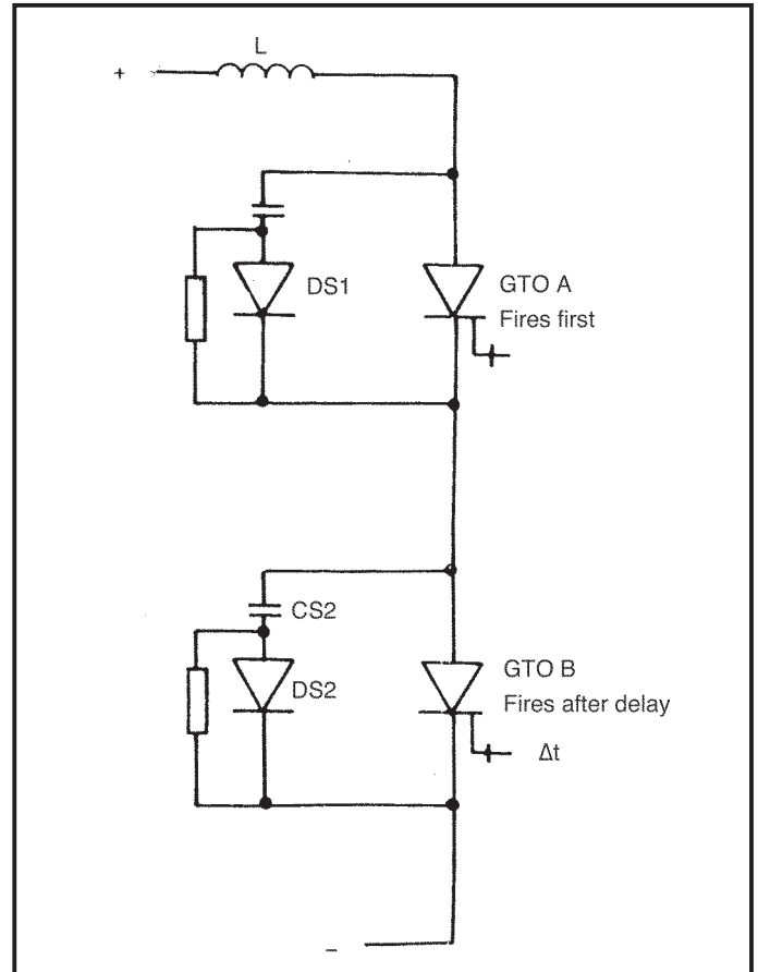
Fig. 1 GTOs in series with snubber networks
