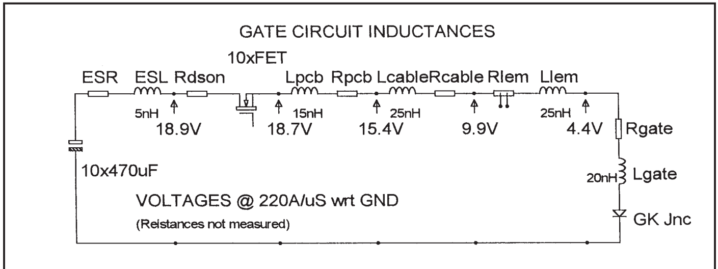
Fig. 4 Loop inductance and dynamic resistance
