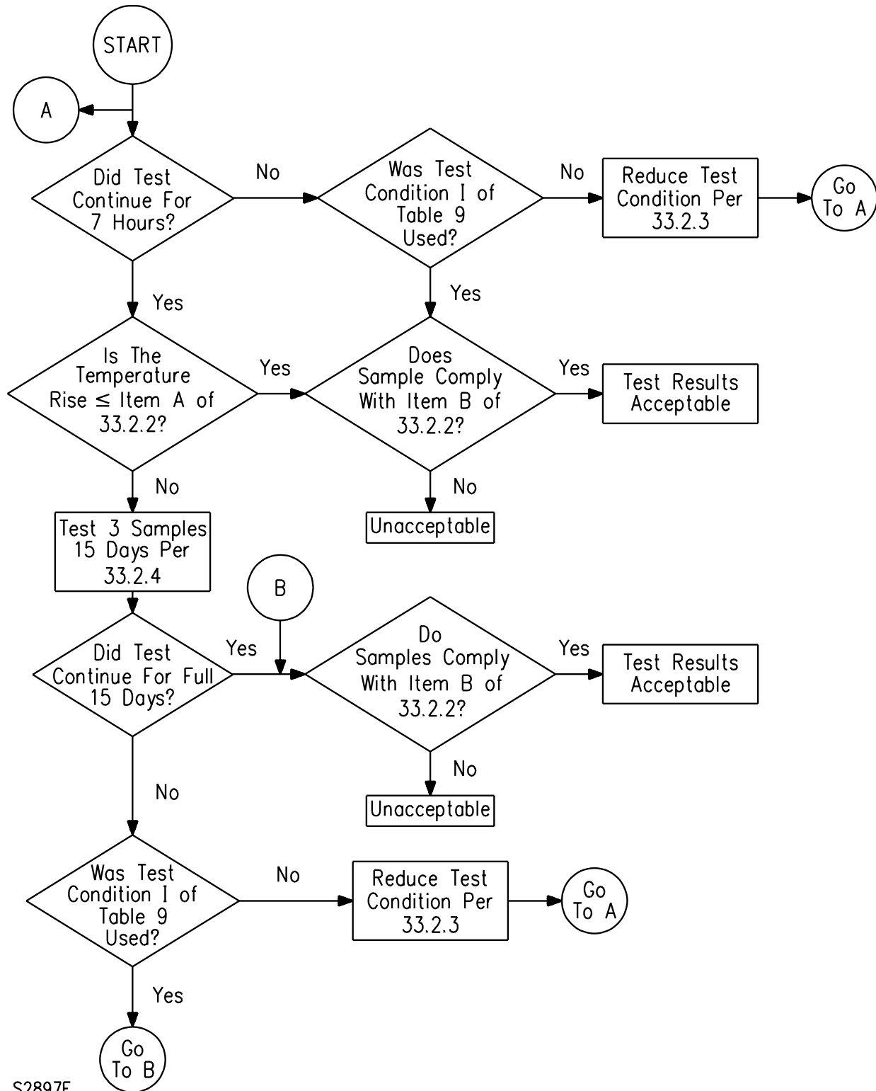
Figure 1 Overload heating test flow chart (See Clauses 33.2.1 and 33.2.3)
