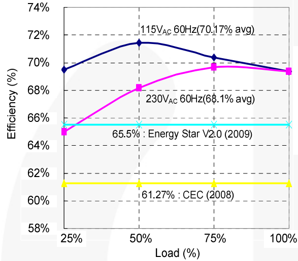
Figure 30. Measured Efficiency
