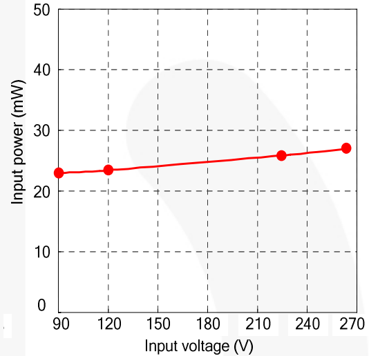
Figure 31. Standby Power
