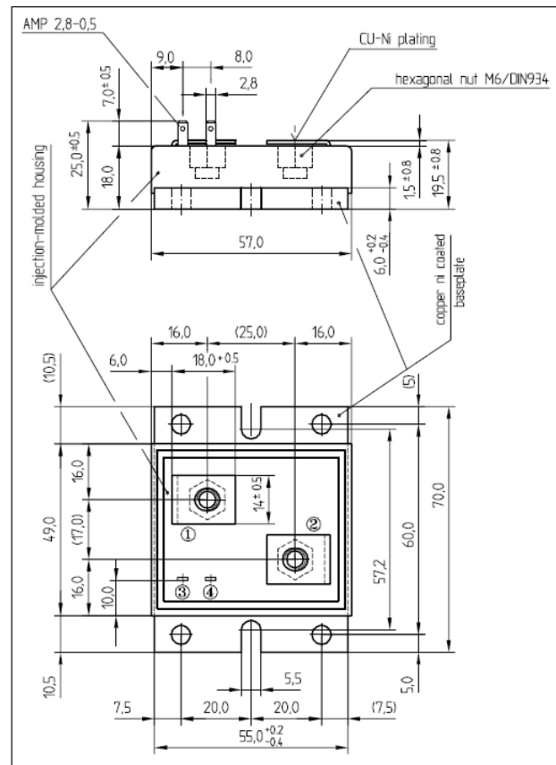
dimensions ( mm )
