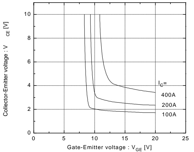
Collector-Emittter vs. Gate-Emittter voltage T_j=125^\circ\text{C}
