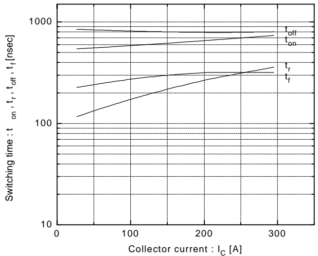
Switching time vs. Collector current V_{CC}=300\text{V}, R_G=9.1\Omega, V_{GE}=\pm 15\text{V}, T_j=125^\circ\text{C}
