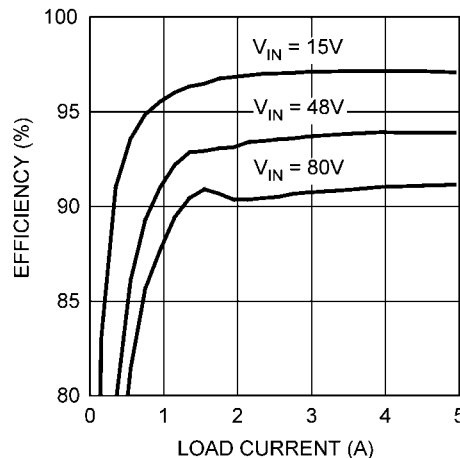
FIGURE 2. Efficiency with 10 µH Pulse Inductor
