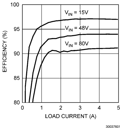
FIGURE 1. Efficiency with 10 µH Gowanda Inductor
