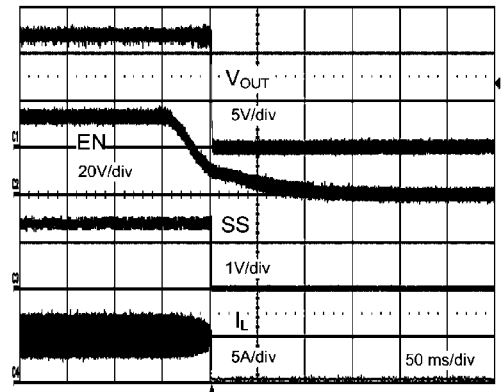
FIGURE 13. Start-up into Active Load at 48V IN
