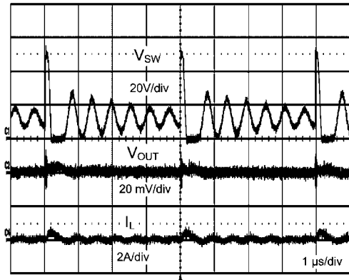
FIGURE 10. Discontinuous Operation using Diode Emulation Mode at 48V IN with JMP1 Installed
