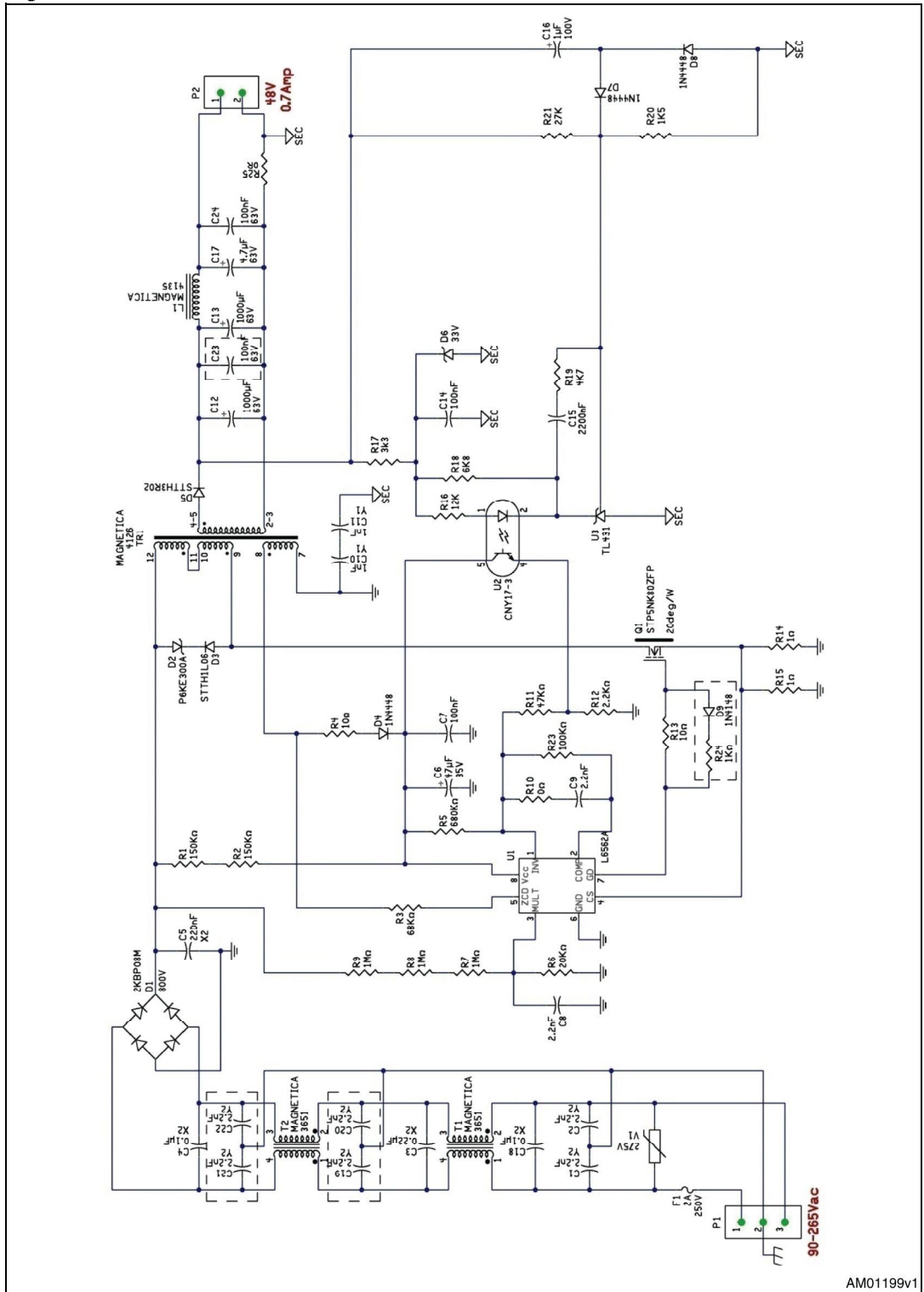
Figure 2. EVL6562A-35WFLB demonstration board: electrical schematic
