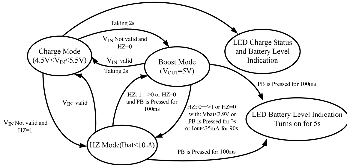
ACT2801 System Operation Flow Chart
