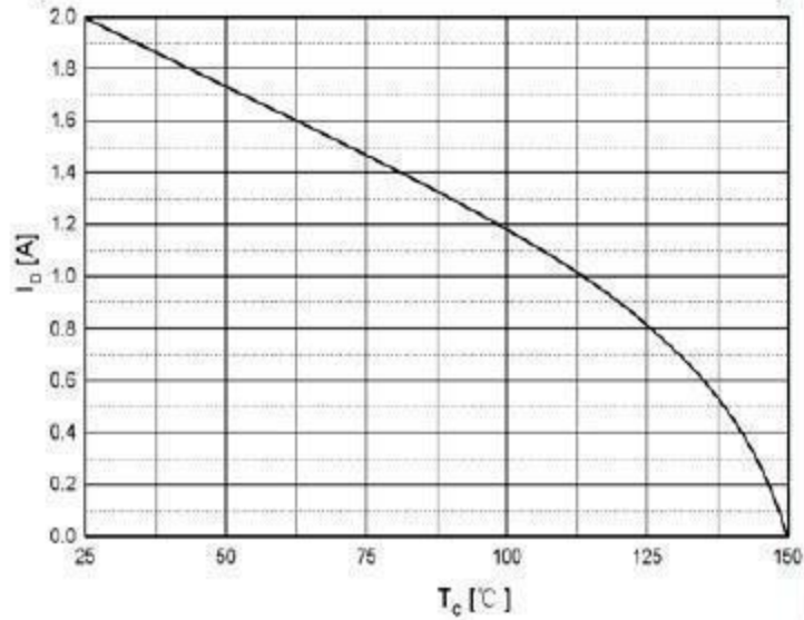
Maximum Drain Current vs. Case Temperature
