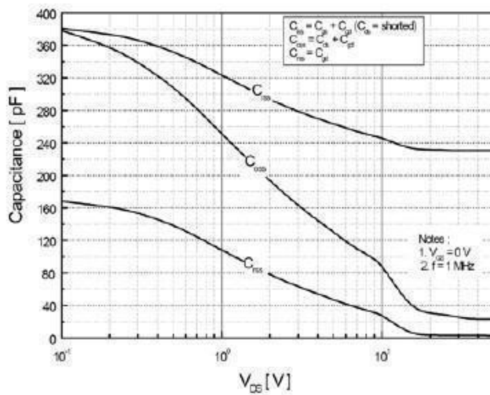
Capacitance Characteristics
