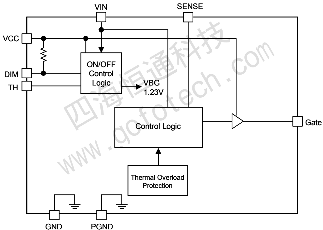
Fig. 3 Block Diagram of G2605
