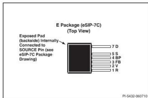
Figure 3. Pin Configuration.
