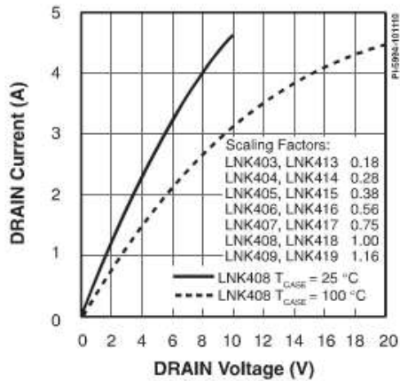
Figure 16. Drain Current vs. Drain Voltage.
