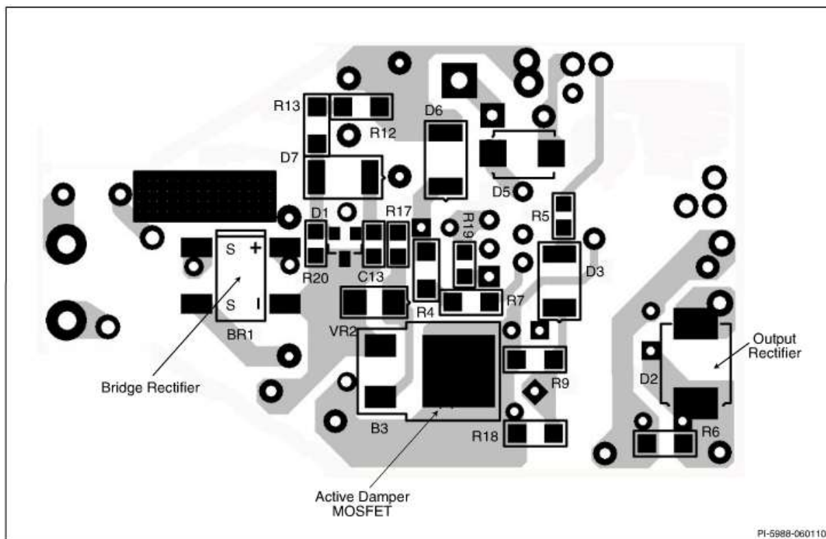
Figure 12. RD-193 7 W Layout Example, Bottom Layer.
