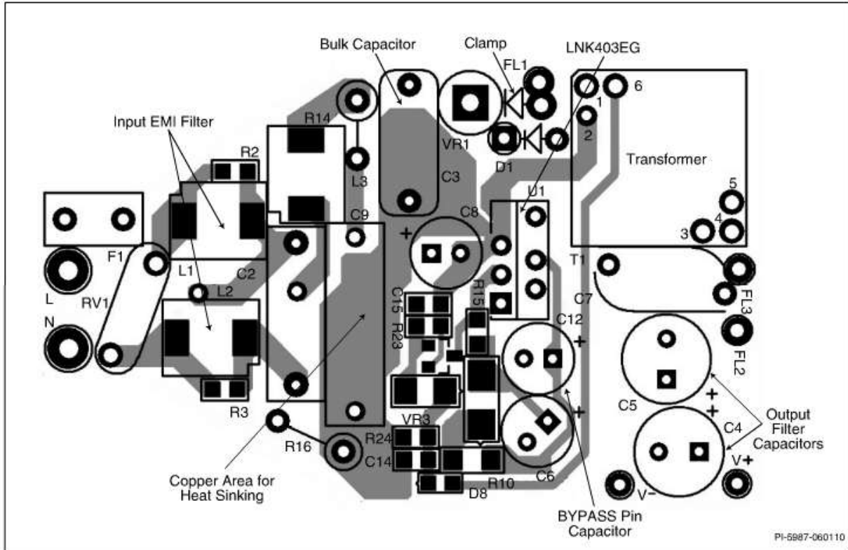
Figure 11. RD-193 7 W Layout Example, Top Layer.
