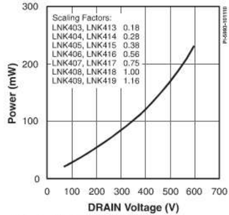
Figure 15. Power vs. Drain Voltage.
