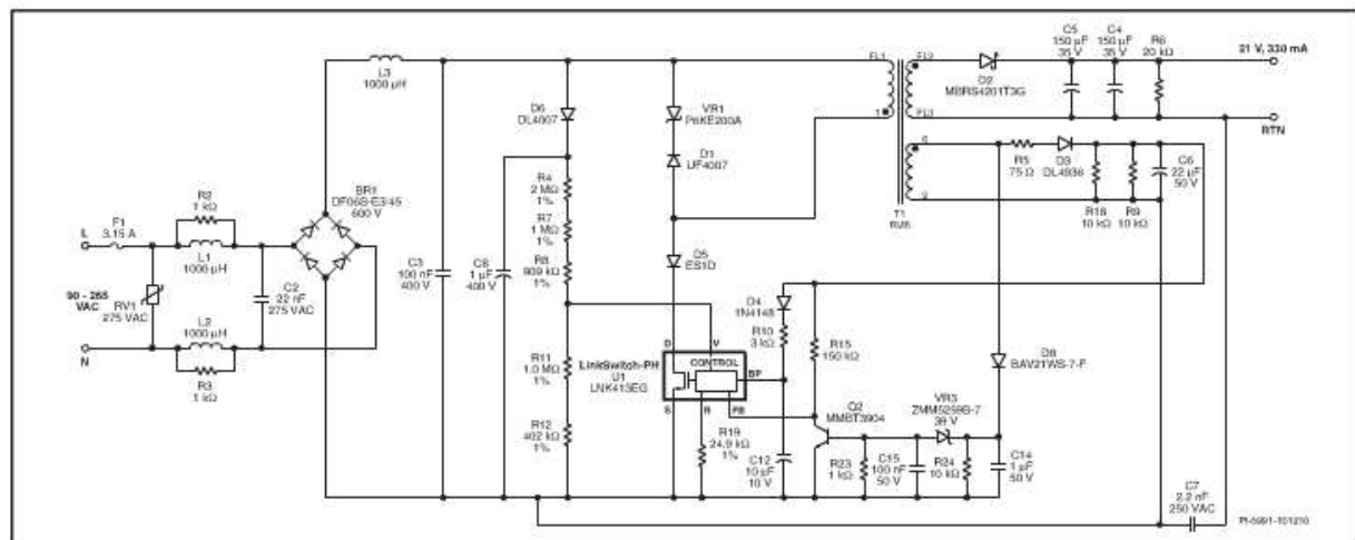
Figure 7. Schematic of an Isolated, Non-Dimmable, High Power Factor, Universal Input, 7 W LED Driver.
