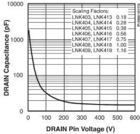
Figure 14. Drain Capacitance vs. Drain Pin Voltage.
