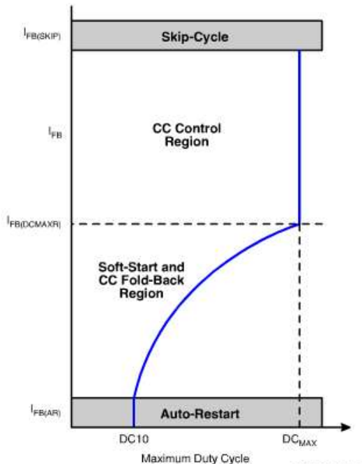
Figure 4. FEEDBACK Pin Current Characteristic.
