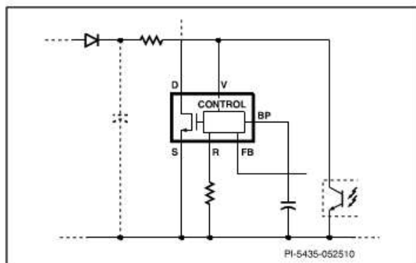
Figure 5. Remote ON/OFF VOLTAGE MONITOR pin Control
