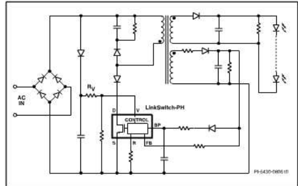
Figure 1. Typical Application Schematic.
