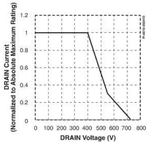
Figure 17. Maximum Allowable Drain Current vs. Drain Voltage.
