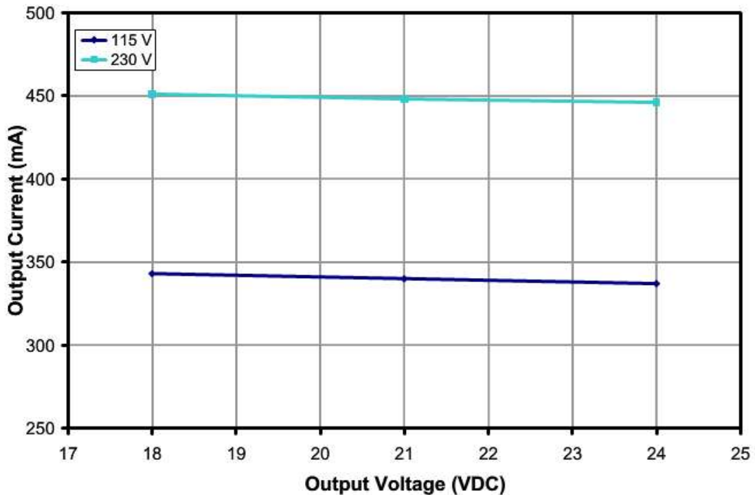
Figure 8 – Voltage and Line Regulation, Room Temperature.
