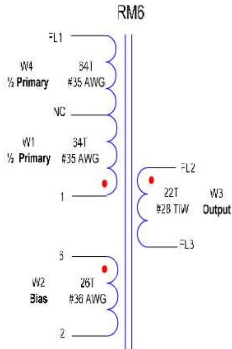
Figure 5 – Transformer Electrical Diagram.
