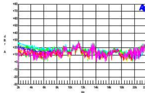
Figure 42 – 2 kHz – 22 kHz.
