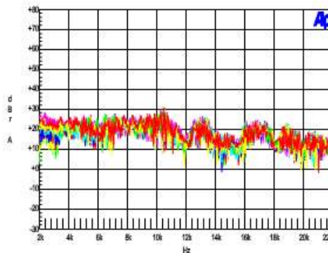
Figure 44 – 2 kHz – 22 kHz.
