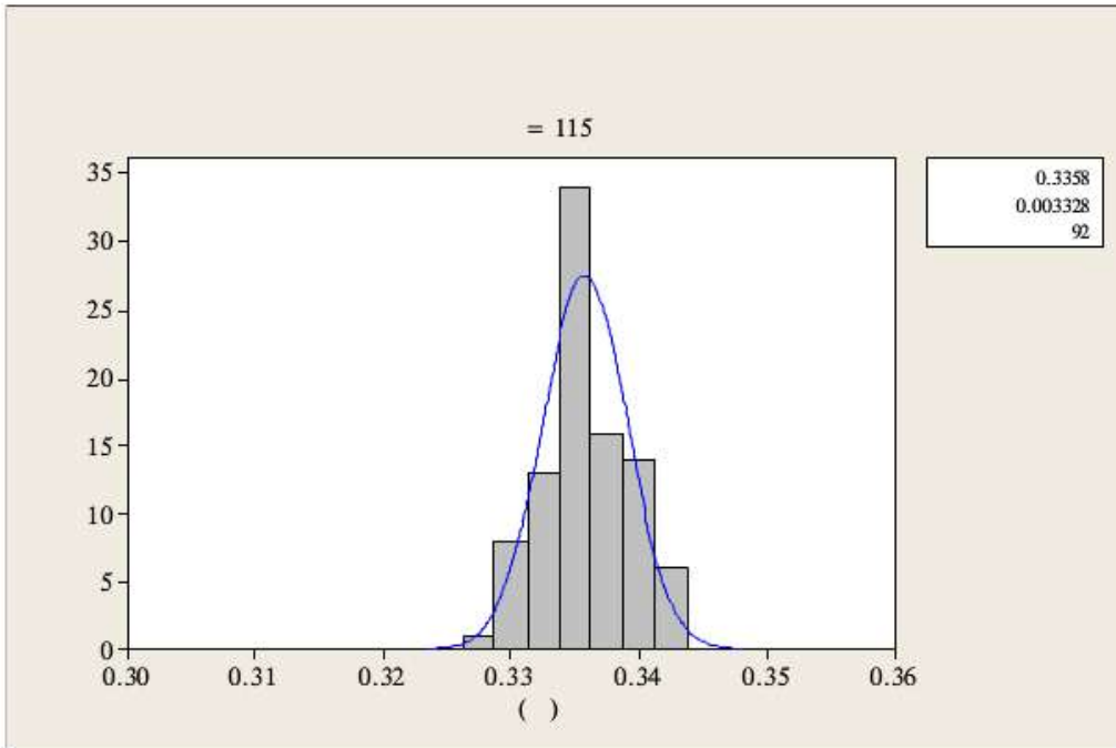
Figure 40 – Production Variation of I OUT at 115 VAC.
