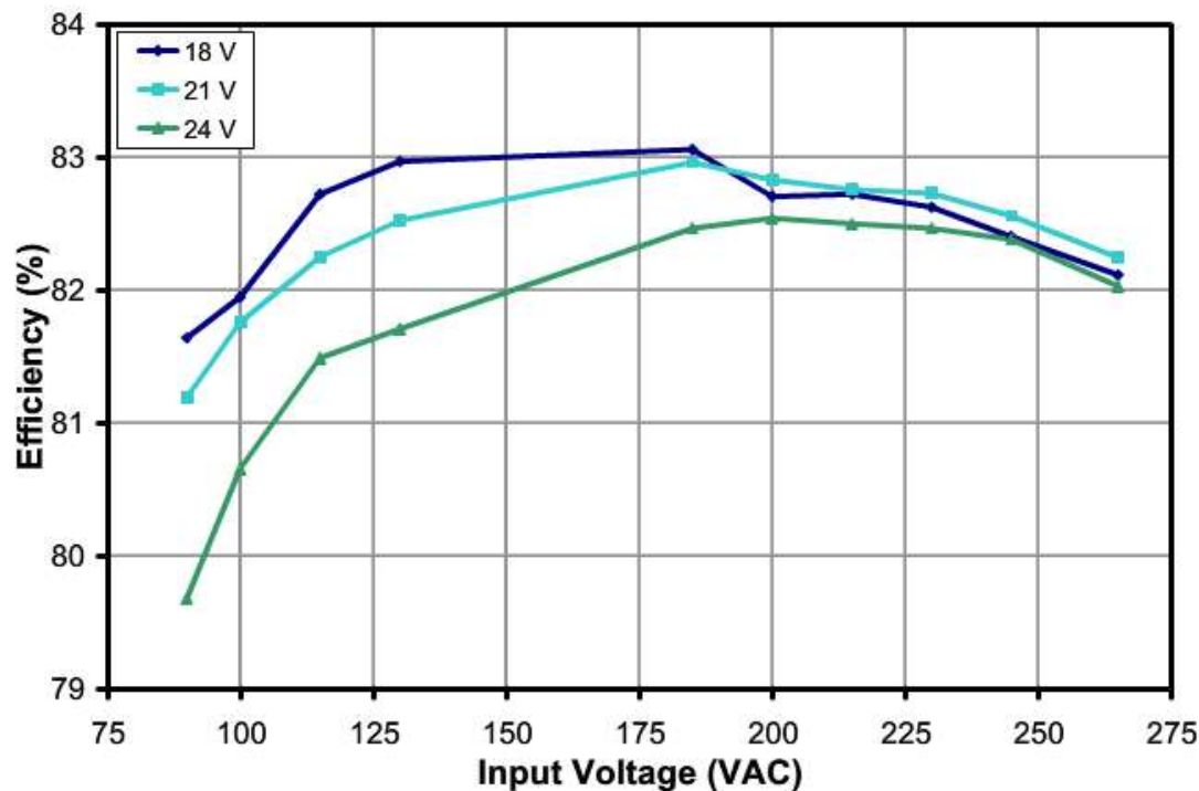
Figure 7 – Efficiency vs. Input Voltage, Room Temperature.
