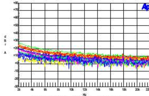
Figure 41 – 2 kHz – 22 kHz.
