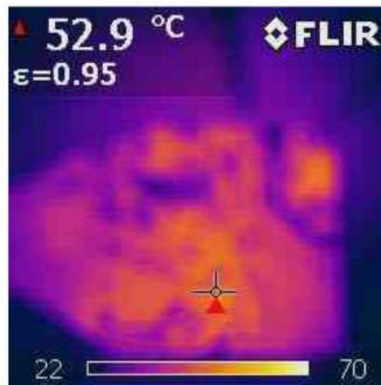
Figure 14 – Bottom Side.
