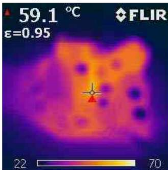
Figure 13 – Top Side.
