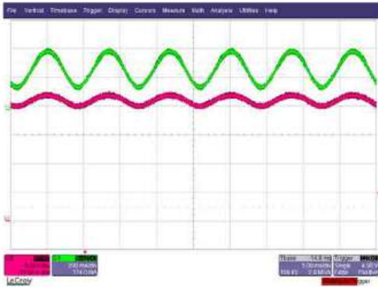
Figure 21 – 90 VAC, Full Load. Upper: I_{RIPPLE} , 0.2 A / div. Lower: V_{OUTPUT} 5 V, 5 ms / div.
