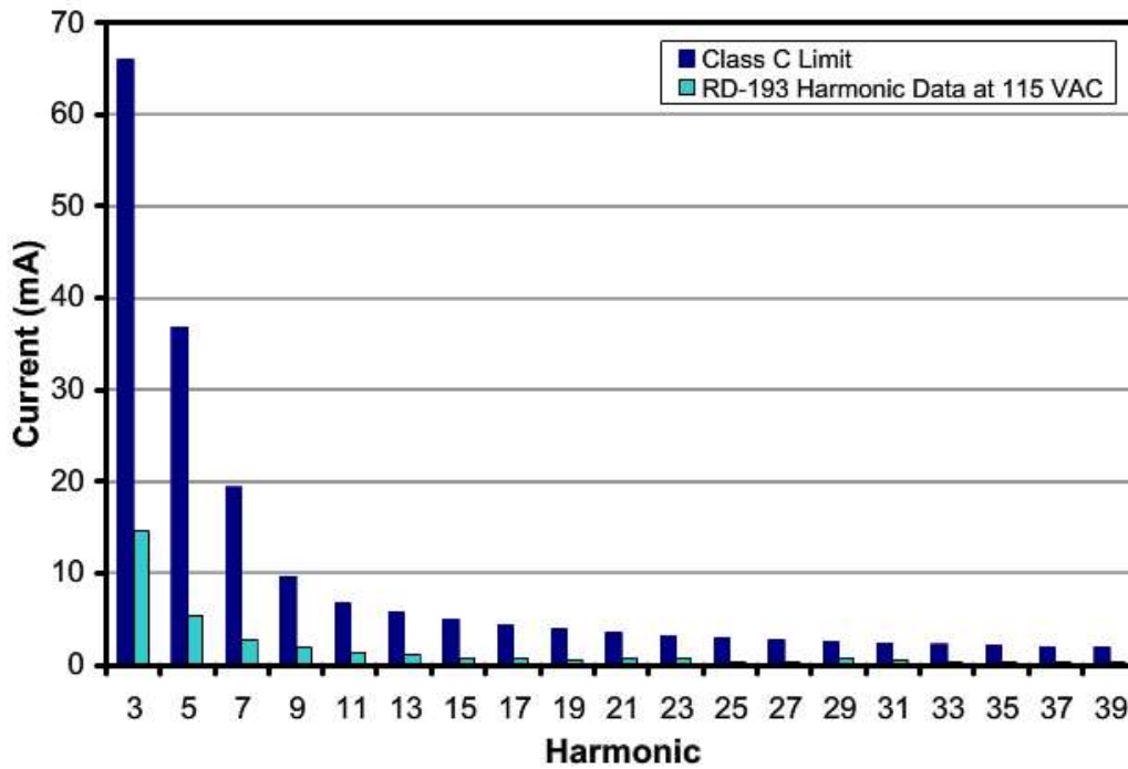
Figure 15 – 115 VAC Harmonic, Room Temperature, Full Load.
