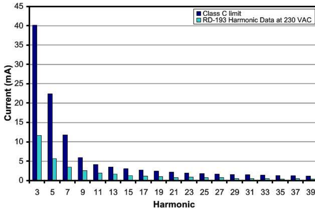
Figure 16 – 230 VAC Harmonic, Room Temperature, Full Load.
