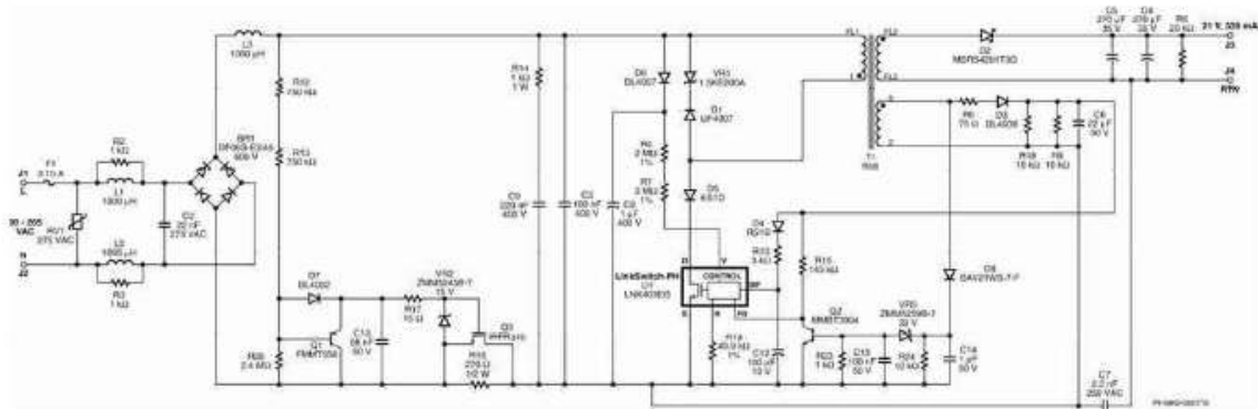
Figure 3 – Schematic.
