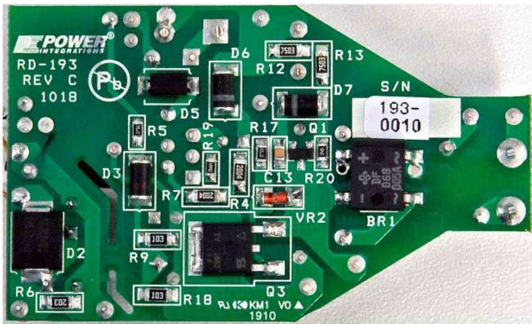
Figure 2 – Populated Circuit Board Photograph (Bottom View).
