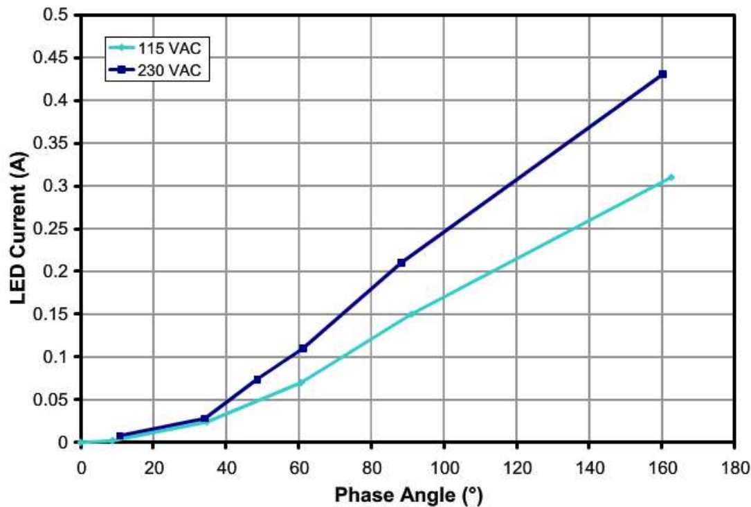
Figure 29 – Input Phase vs. Output Current.
