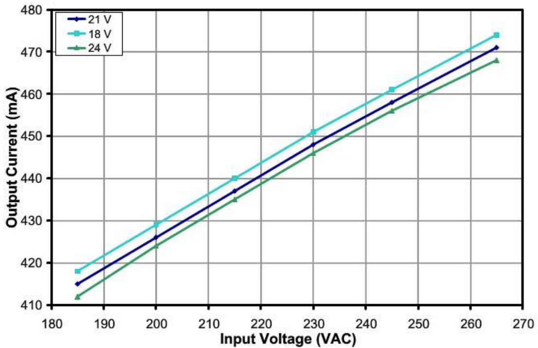
Figure 10 – High Line Regulation, Room Temperature, Full Load.
