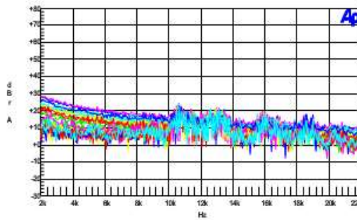
Figure 43 – 2 kHz – 22 kHz.
