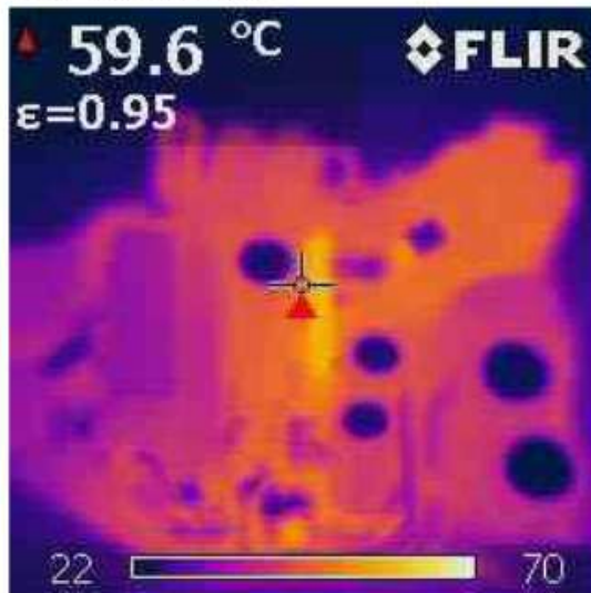
Figure 11 – Top Side.
