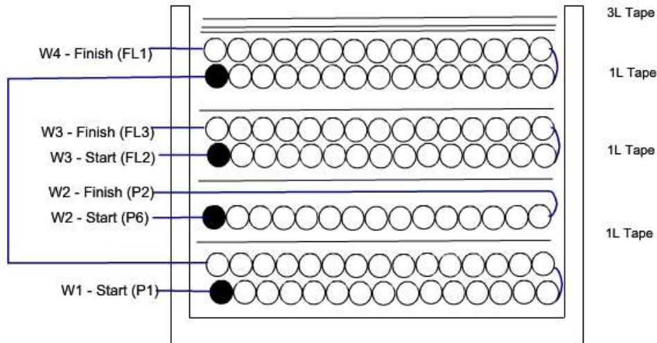
Figure 6 – Transformer Build Diagram.
