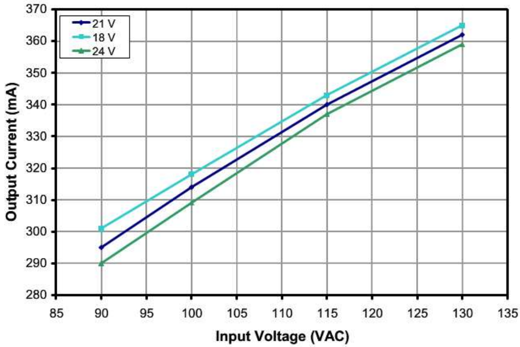
Figure 9 – Low Line Regulation, Room Temperature, Full Load.
