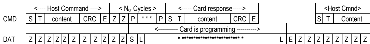
Figure 4-24. Stop Transmission Received After Last Data Block. Card becomes Busy
